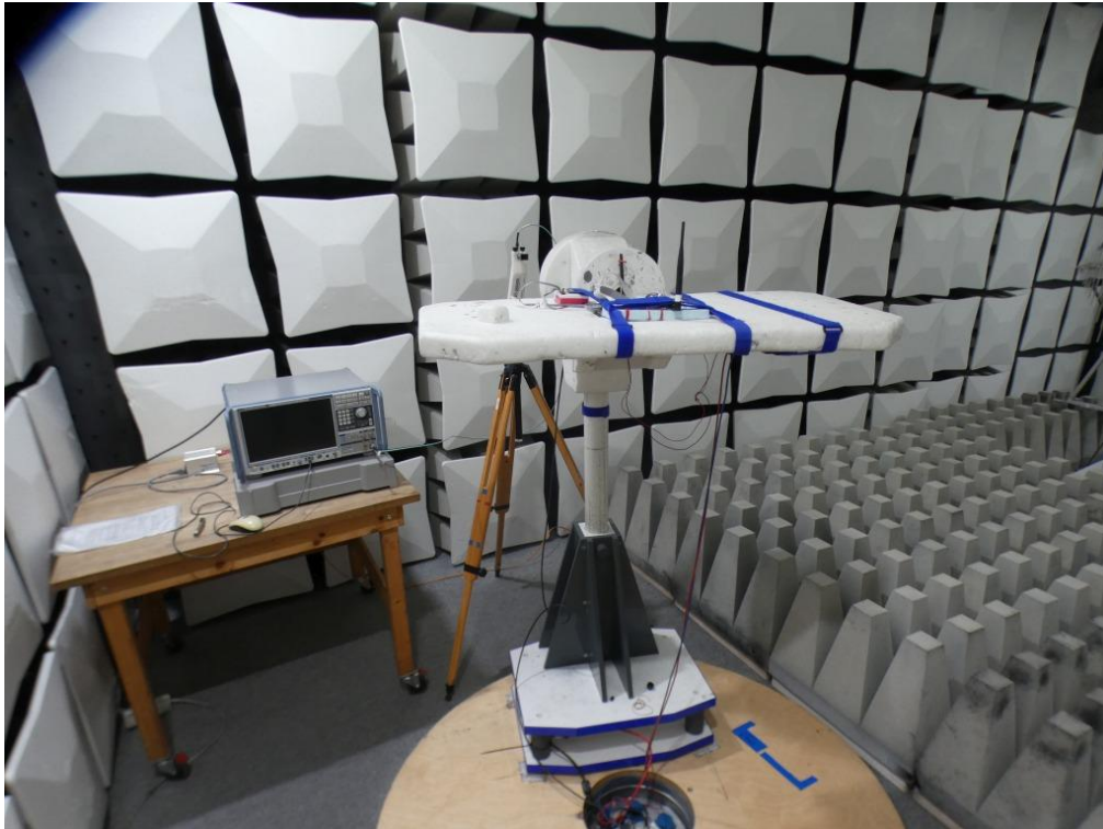
Photo 7: Test setup for radiated measurements above 26 GHz
