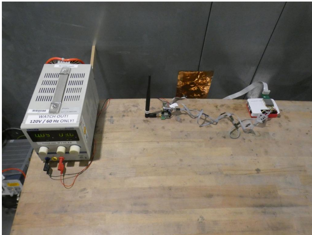
Photo 1: AC Conducted Emissions
