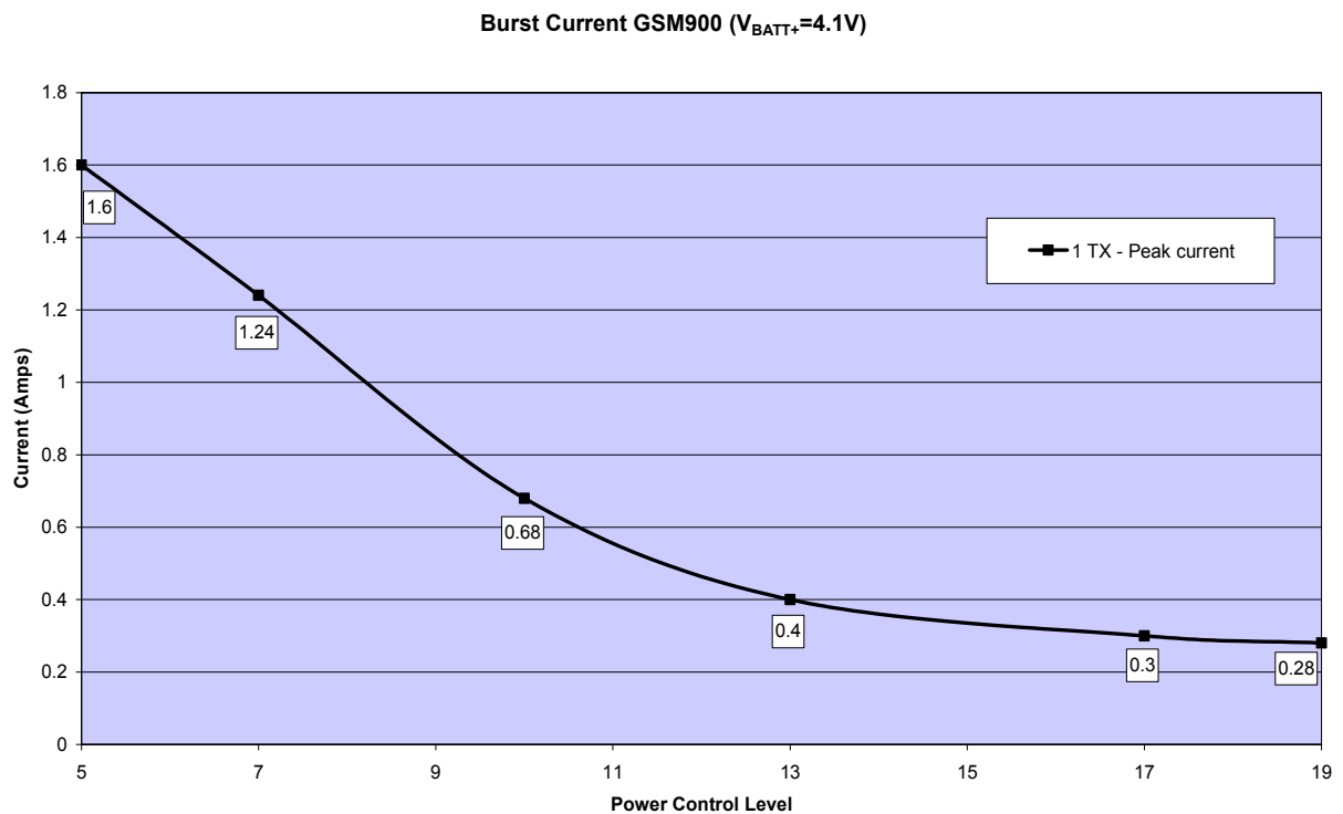
Figure 44: Peak current consumption during transmit burst in EGSM 900 network
