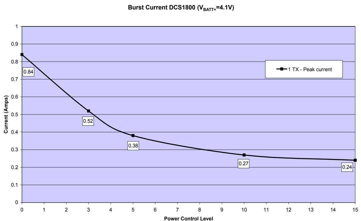
Figure 45: Peak current consumption during transmit burst in GSM 1800 network
