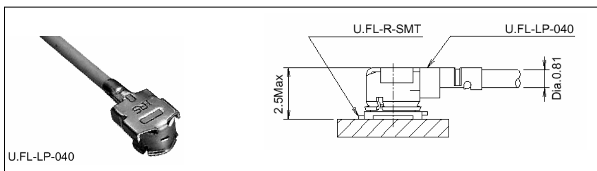
Figure 37: U.FL-R-SMT connector with U.FL-LP-040 plug
