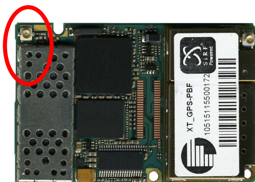
Figure 31: U.FL-R-SMT connector
