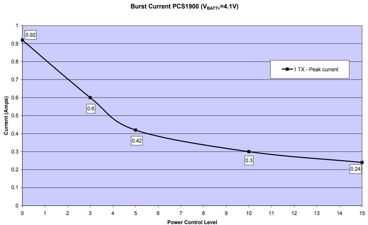
Figure 46: Peak current consumption during transmit burst in GSM 1900 network
