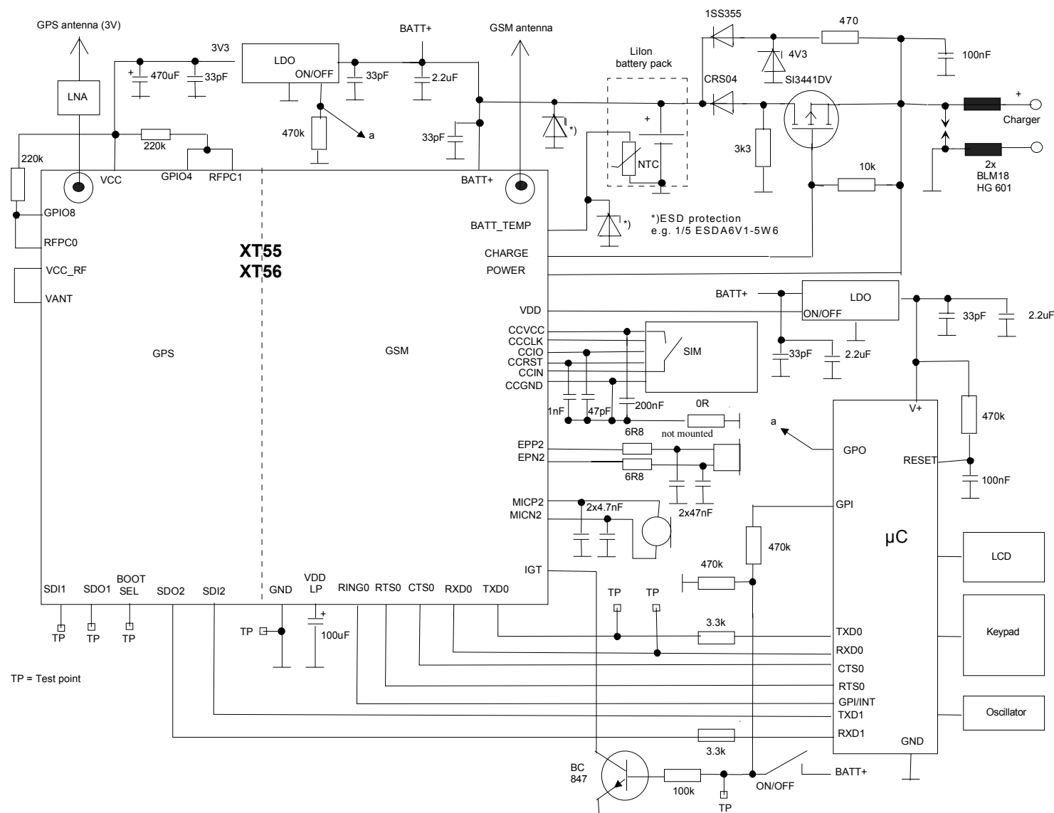
Figure 58: XT55/56 tracking phone with external \mu C (example application)
