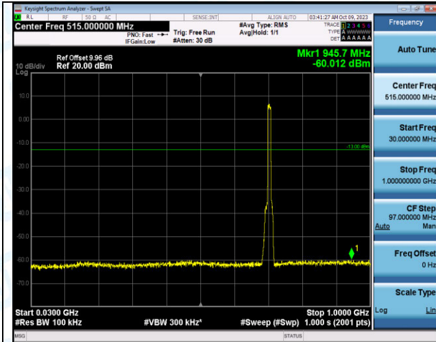
Band12_10MHz_QPSK_23130_50RB#0_30~1000_30~1000
