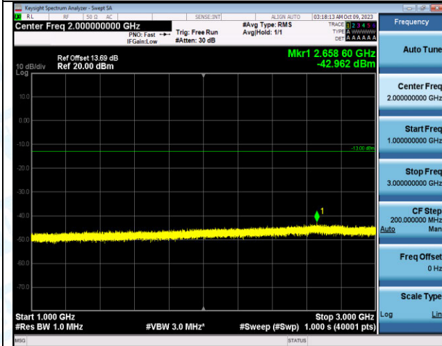
Band12_10MHz_16QAM_23095_1RB#49_1000~3000_1000~3000
