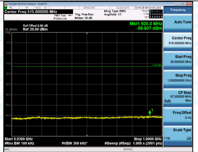
Band12_10MHz_QPSK_23095_50RB#0_30~1000_30~100
