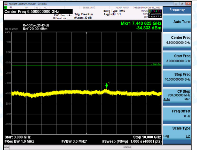
Band12_10MHz_16QAM_23130_1RB#0_3000~10000_30 00~10000
