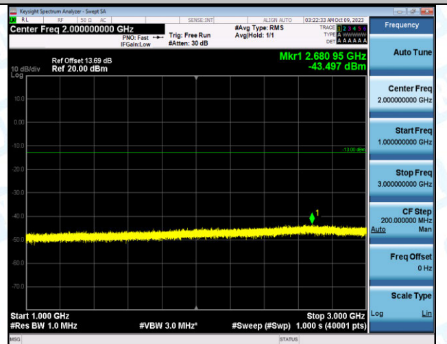
Band12_10MHz_QPSK_23130_1RB#49_1000~3000_1000 ~3000
