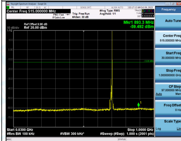
Band12_10MHz_QPSK_23095_1RB#49_30~1000_30~1000
