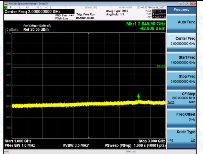
Band12_10MHz_QPSK_23060_50RB#0_1000~3000_1000~3000
