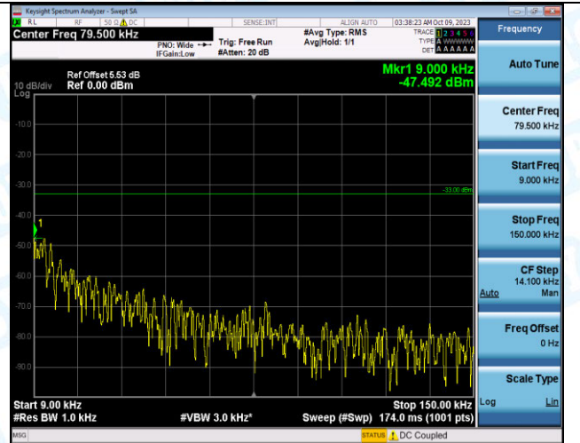
Band12_10MHz_16QAM_23130_1RB#49_0.009~0.15_0.0 09~0.15
