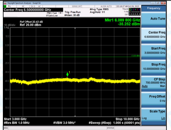
Band12_10MHz_16QAM_23095_1RB#49_3000~10000_3000~10000
