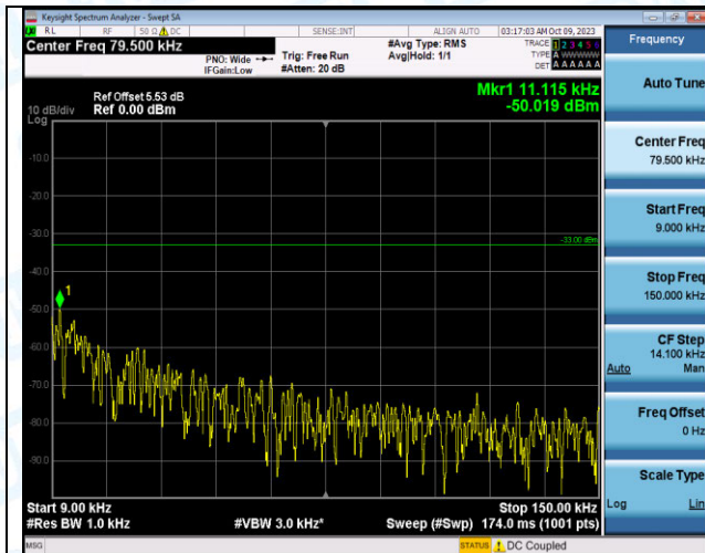
Band12_10MHz_QPSK_23095_1RB#49_0.009~0.15_0.09~0.15
