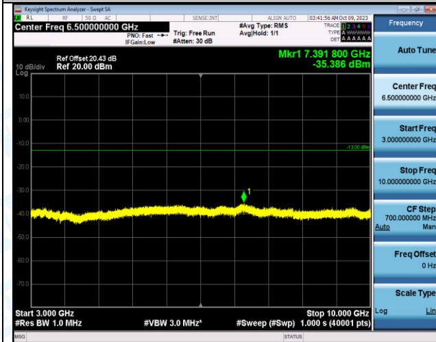
Band12_10MHz_QPSK_23130_50RB#0_3000~10000_3000~10000
