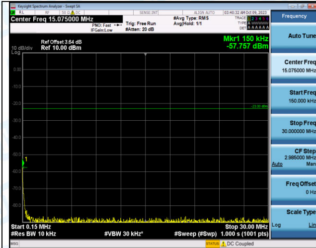
Band12_10MHz_QPSK_23095_50RB#0_0.15~30_0.15~3
