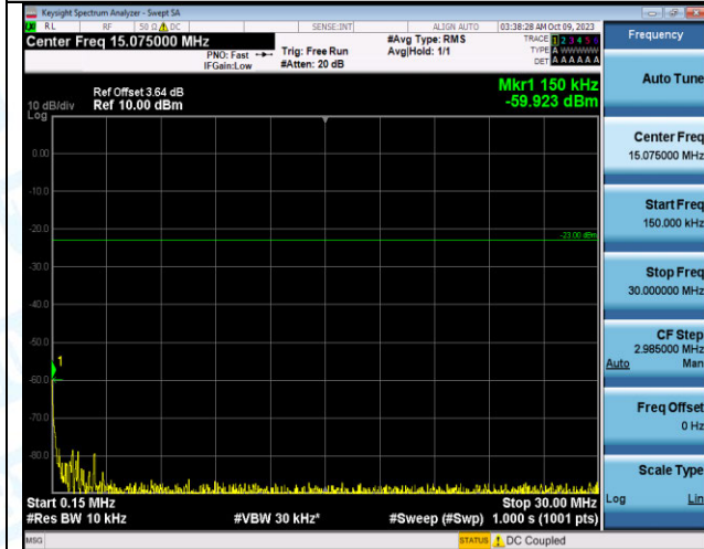
Band12_10MHz_16QAM_23130_1RB#49_0.15~30_0.15~30 30
