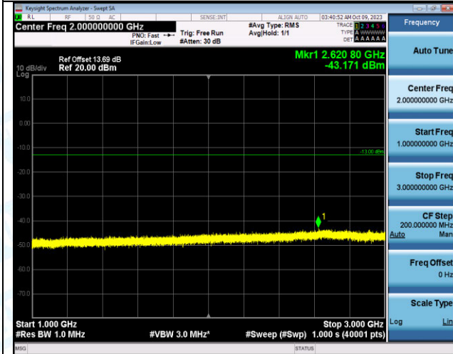
Band12_10MHz_QPSK_23095_50RB#0_1000~3000_1000~3000
