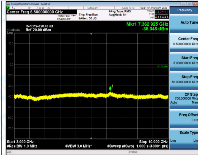
Band12_10MHz_QPSK_23095_1RB#0_3000~10000_300 0~10000
