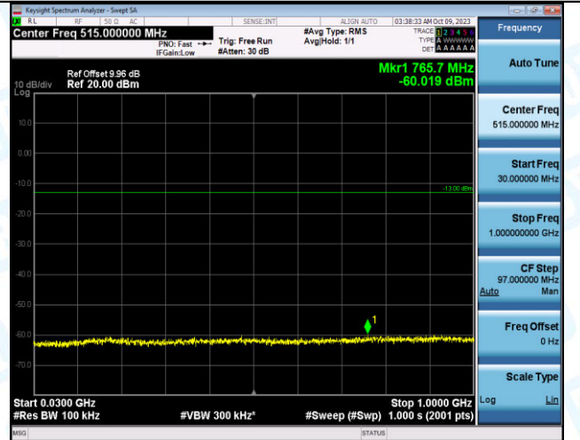
Band12_10MHz_16QAM_23130_1RB#49_30~1000_30~1000 000
