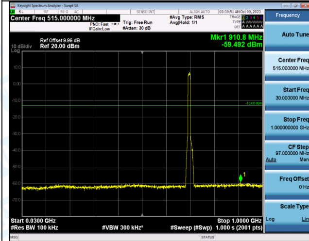
Band12_10MHz_QPSK_23060_50RB#0_30~1000_30~1000
