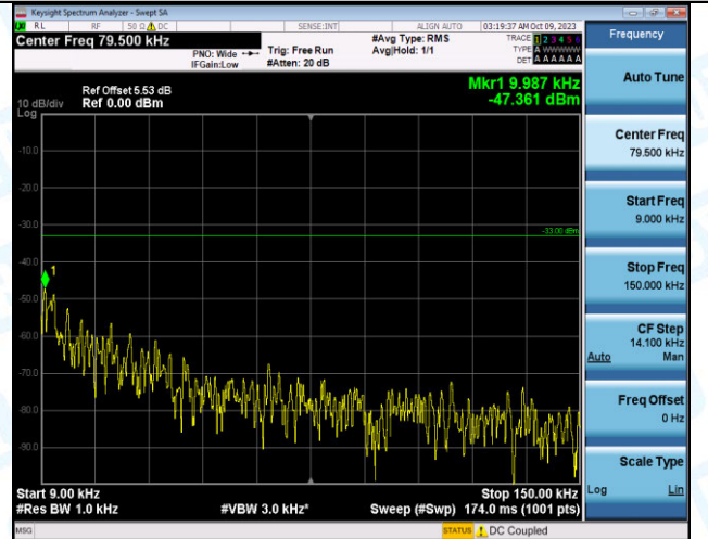
Band12_10MHz_16QAM_23130_1RB#0_0.009~0.15_0.009~ 9~0.15
