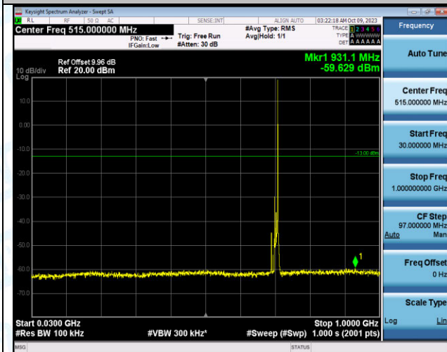
Band12_10MHz_QPSK_23130_1RB#49_30~1000_30~10 00
