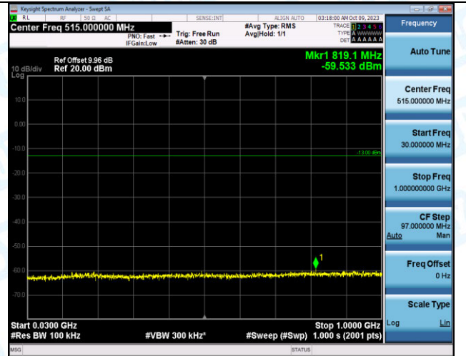
Band12_10MHz_16QAM_23095_1RB#49_30~1000_30~1000
