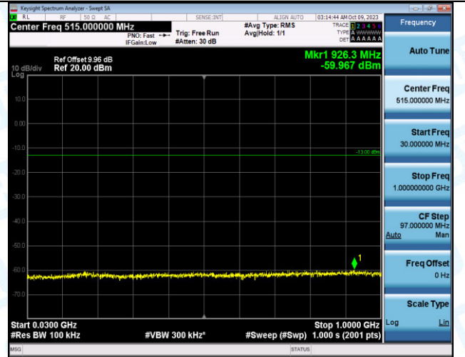
Band12_10MHz_16QAM_23095_1RB#0_30~1000_30~10 00
