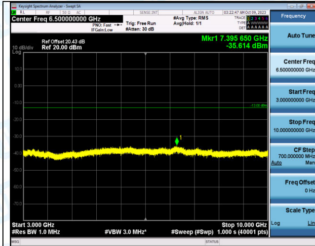
Band12_10MHz_QPSK_23130_1RB#49_3000~10000_30 00~10000
