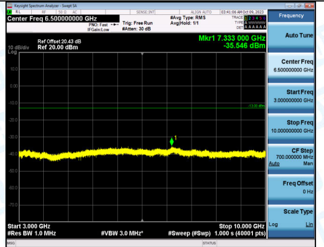
Band12_10MHz_QPSK_23095_50RB#0_3000~10000_3000~10000
