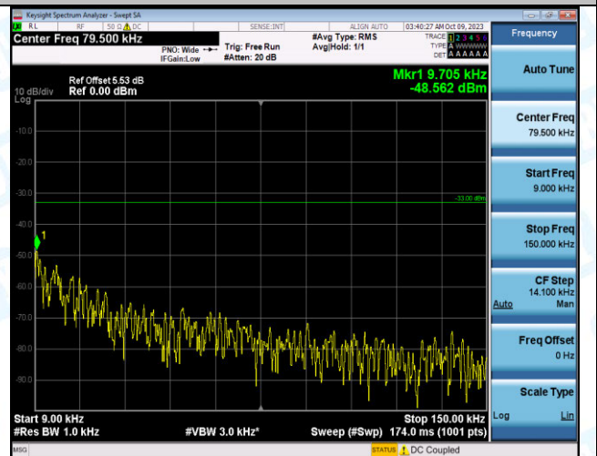
Band12_10MHz_QPSK_23095_50RB#0_0.009~0.15_0.009~0.15
