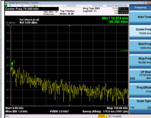
Band12_10MHz_QPSK_23130_1RB#49_0.009~0.15_0.0 09~0.15
