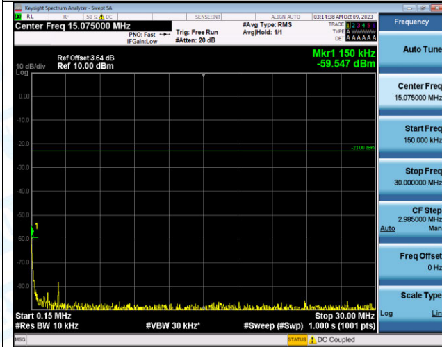
Band12_10MHz_16QAM_23095_1RB#0_0.15~30_0.15~3 0
