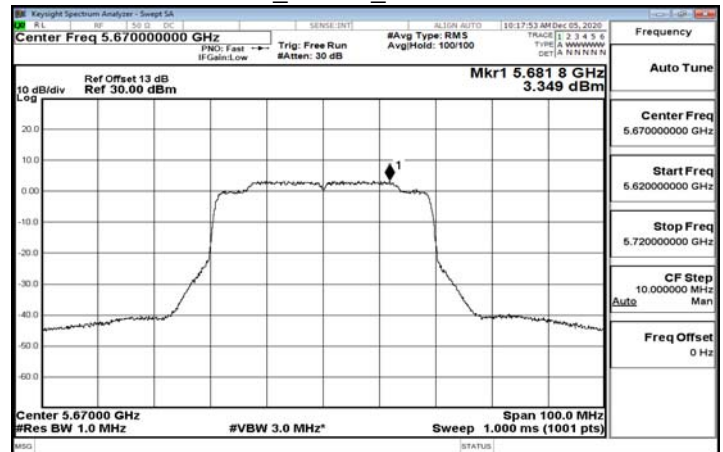
802.11ax_40MHz_5670MHz-5670
