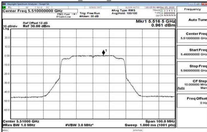
802.11ax_40MHz_5510MHz-5510
