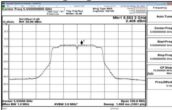
802.11n_40MHz_5550MHz-5550
