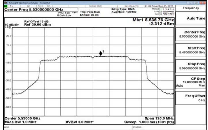
802.11ax_80MHz_5530MHz-5530
