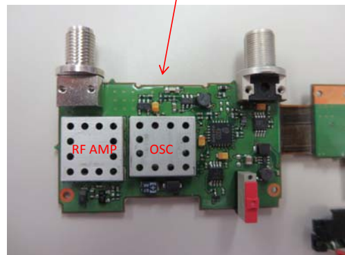
RF Board
