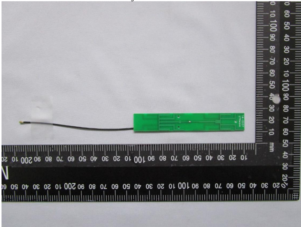
Accessory: AD-509AX Pic 1
