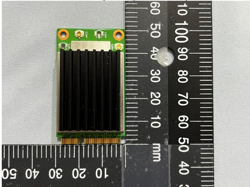
Outview: WPEQ-276AX(With Heatsink) Pic 1
