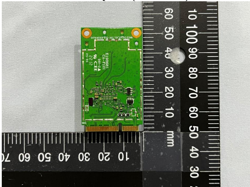
Outview: WPEQ-276AX(With Heatsink) Pic 2
