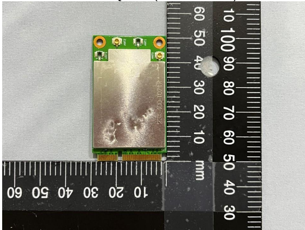
Outview: WPEQ-276AX(Without Heatsink) Pic 1
