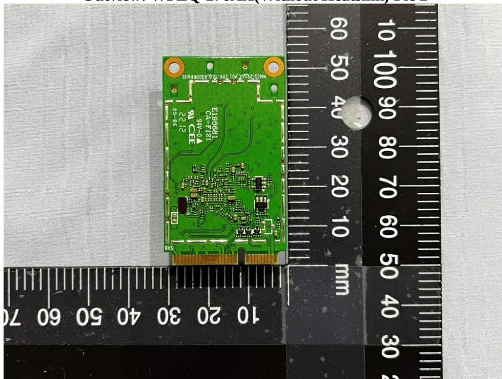
Outview: WPEQ-276AX(Without Heatsink) Pic 2
