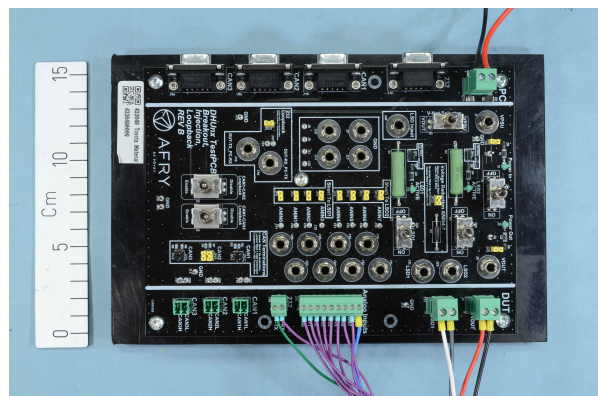
Test Jig
