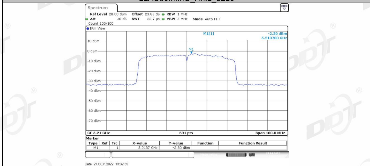
11AC80MIMO Ant2 5210
