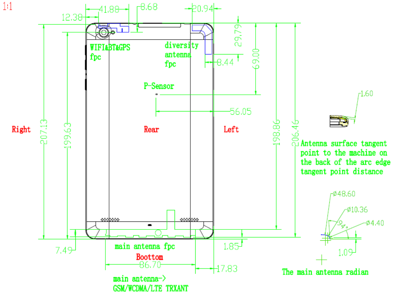
Fig.11.1 EUT Antenna Locations
