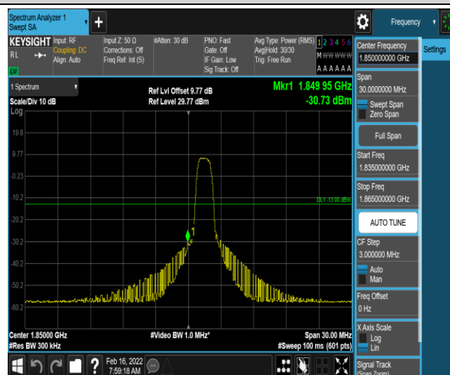
Band25-15MHz-16QAM-26115-6-0-Low--30.73-PASS
