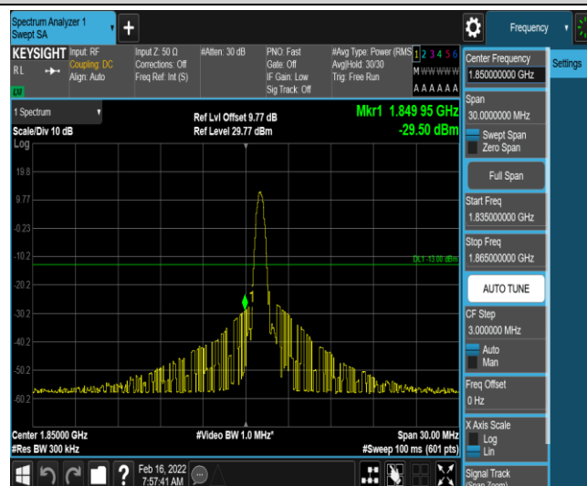
Band25-15MHz-16QAM-26115-1-0-Low--29.50-PASS
