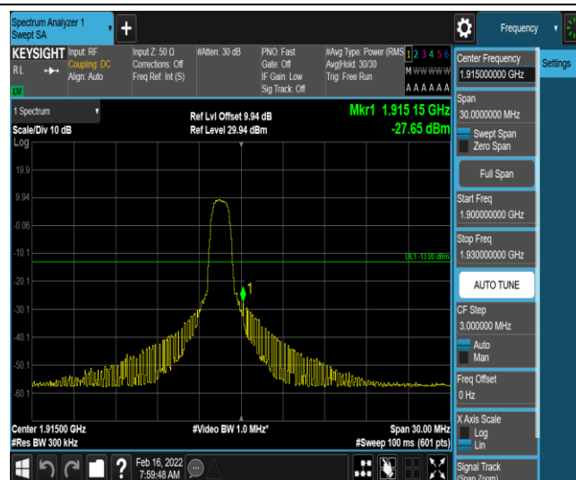
Band25-15MHz-QPSK-26615-6-0-High--27.65-PASS
