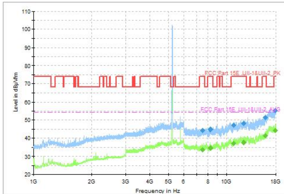
Fig. 55 Transmitter Spurious Emission (802.11n-HT40, CH46 5230MHz, 1GHz-18GHz)
