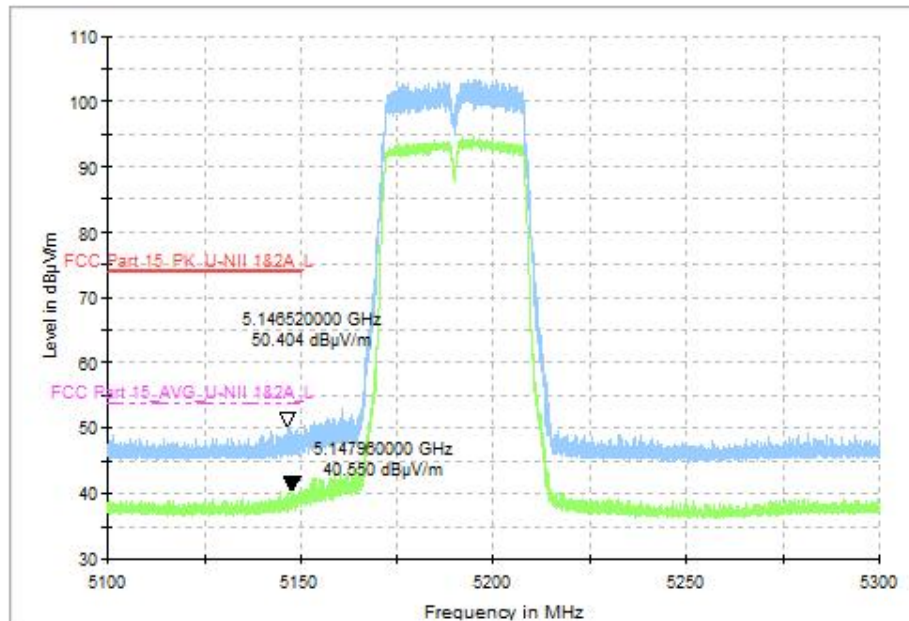
Fig. 31 Band Edges (802.11n-HT40, CH38 5190MHz)
