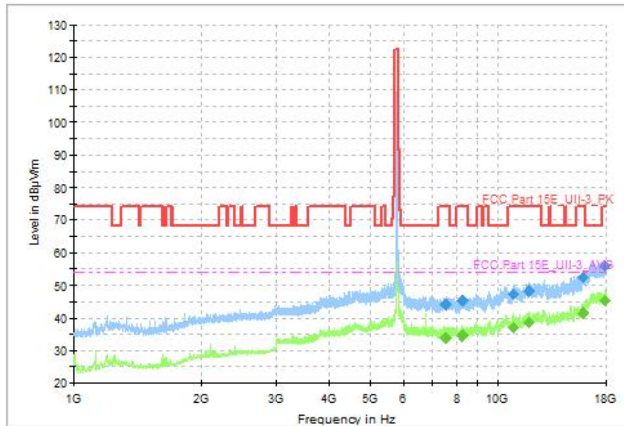
Fig. 57 Transmitter Spurious Emission (802.11n-HT40, CH159 5795MHz, 1GHz-18GHz)
