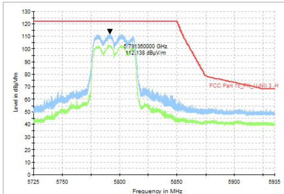
Fig. 41 Band Edges (802.11n-HT40, CH159 5795MHz), MIMO
