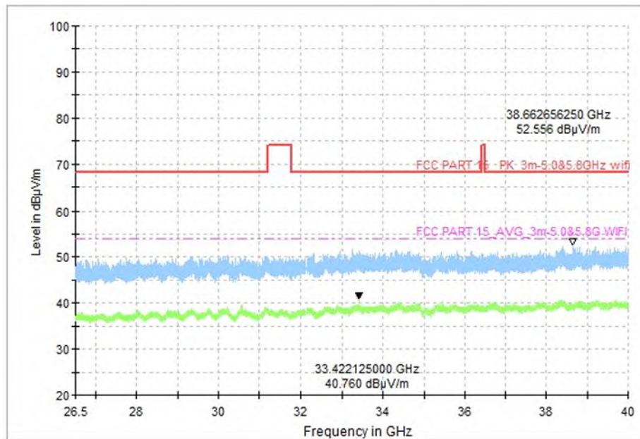
Fig. 81 Transmitter Spurious Emission (DH5 & 802.11ax-HE20, CH0 2402MHz & CH36 5180MHz, 26.5GHz~40GHz)
