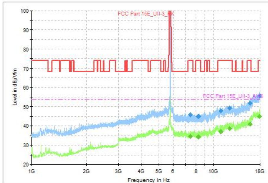
Fig. 59 Transmitter Spurious Emission (802.11ac-VHT80, CH155 5775MHz, 1GHz-18GHz)
