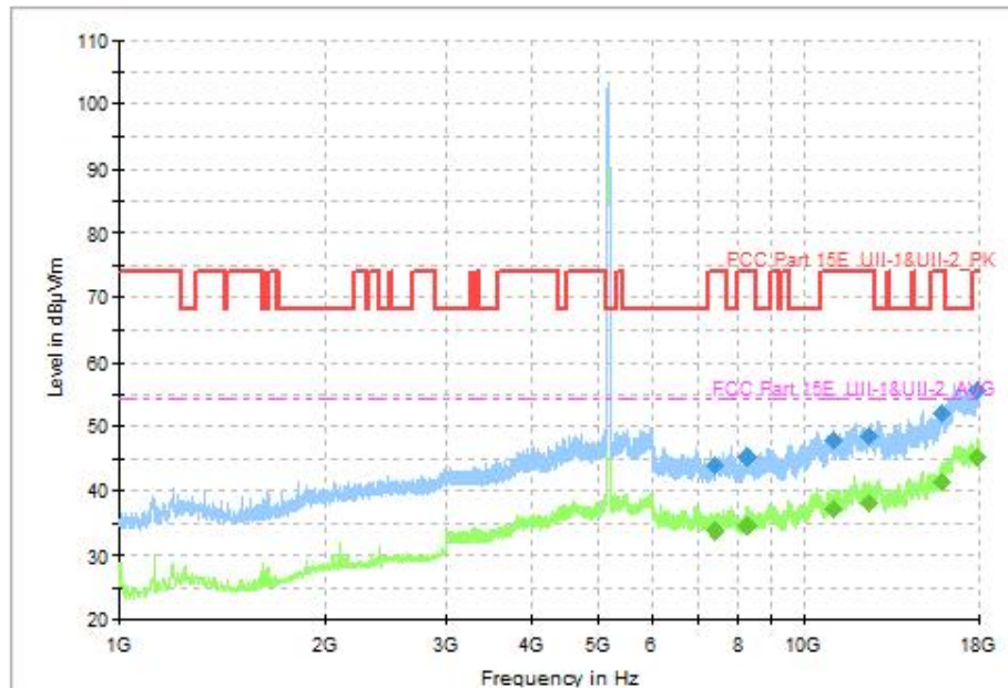
Fig. 54 Transmitter Spurious Emission (802.11n-HT40, CH38 5190MHz, 1GHz-18GHz)
