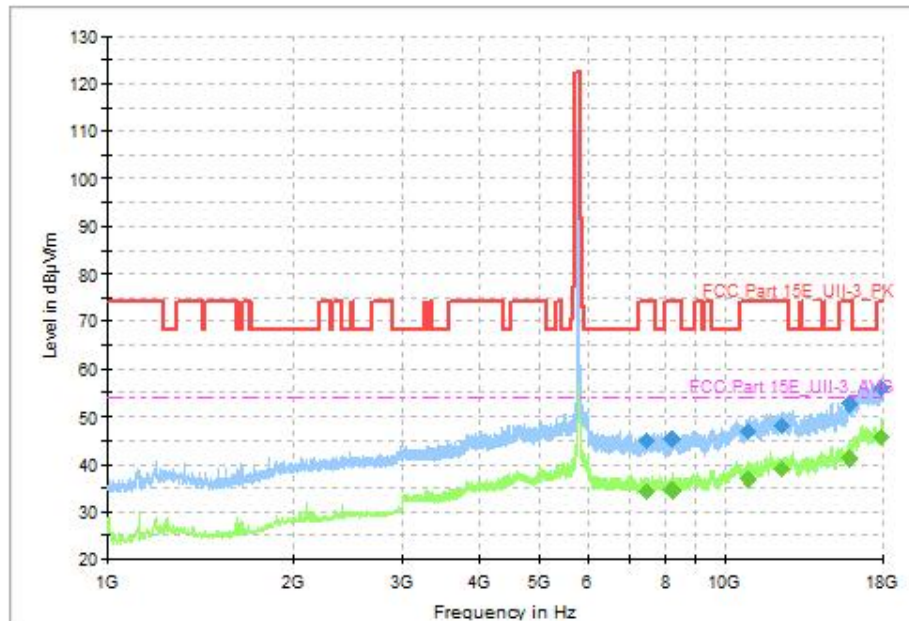
Fig. 72 Transmitter Spurious Emission (802.11n-HT40, CH159 5795MHz, 1GHz-18GHz), MIMO
