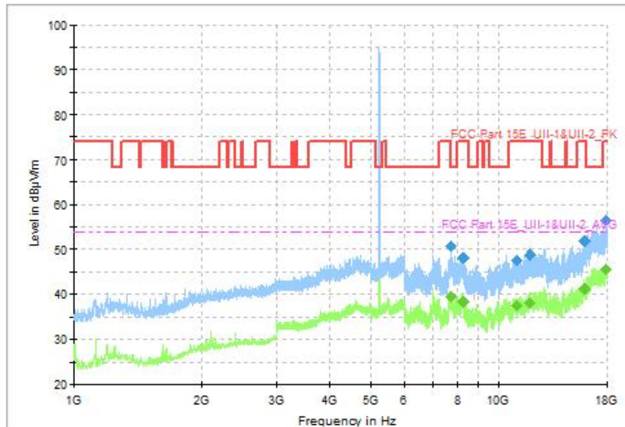
Fig. 46 Transmitter Spurious Emission (802.11ax-HE20, CH48 5240MHz, 1GHz-18GHz)
