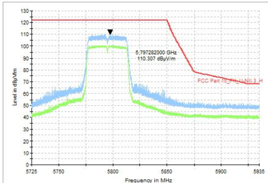
Fig. 33 Band Edges (802.11n-HT40, CH159 5795MHz)
