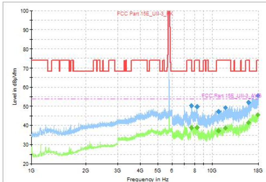
Fig. 48 Transmitter Spurious Emission (802.11ax-HE20, CH157 5785MHz, 1GHz-18GHz)
