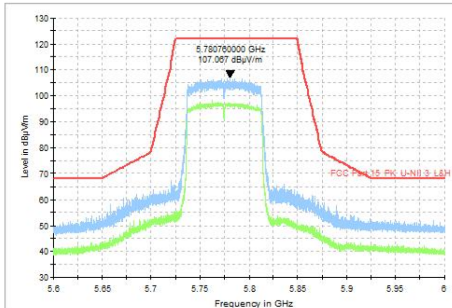
Fig. 35 Band Edges (802.11ac-VHT80, CH155 5775MHz)
