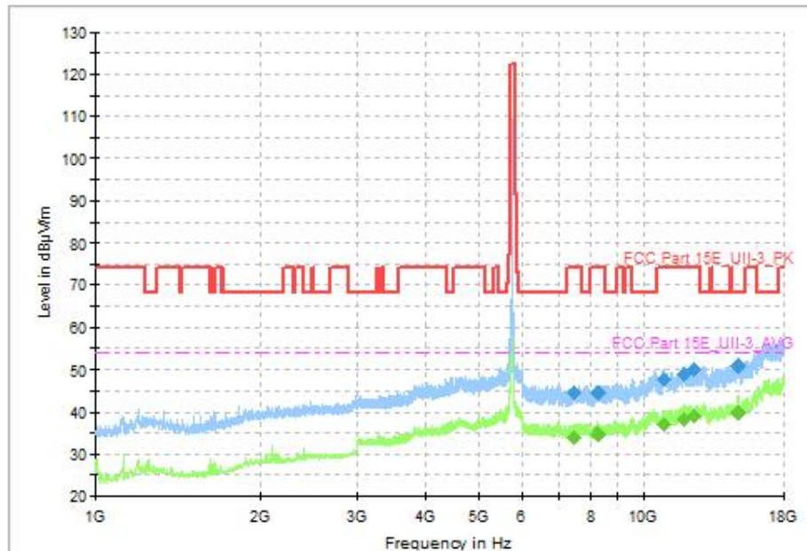
Fig. 56 Transmitter Spurious Emission (802.11n-HT40, CH151 5755MHz, 1GHz-18GHz)
