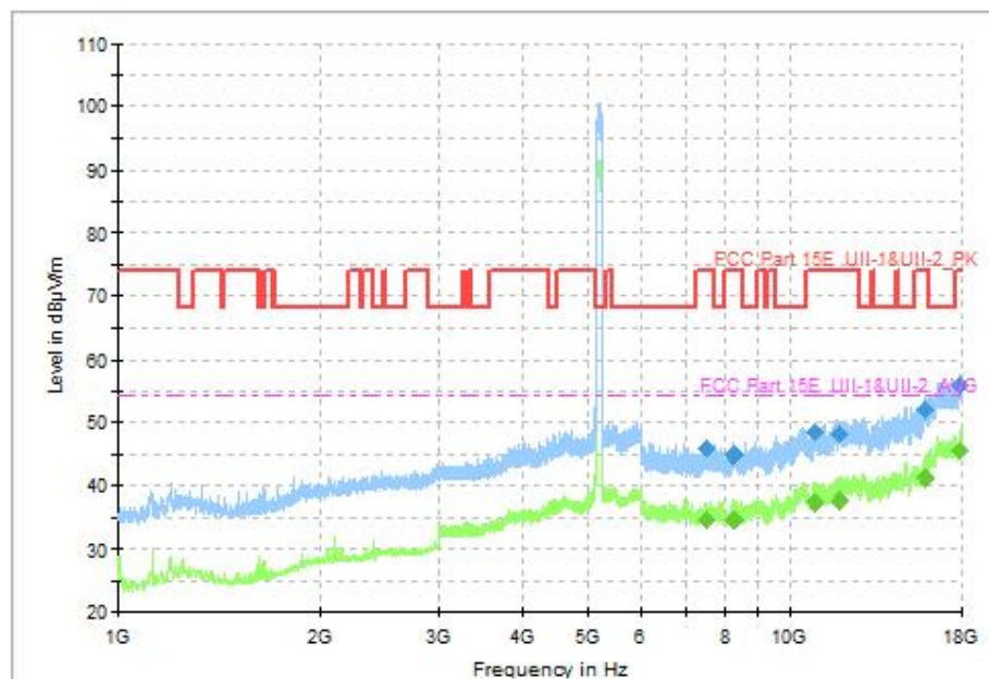
Fig. 73 Transmitter Spurious Emission (802.11ac-VHT80, CH42 5210MHz, 1GHz-18GHz), MIMO
