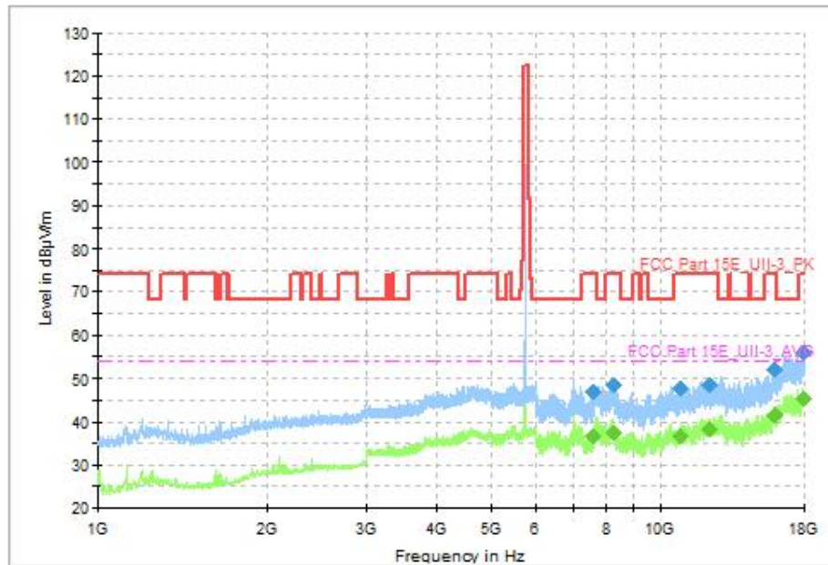
Fig. 47 Transmitter Spurious Emission (802.11ax-HE20, CH149 5745MHz, 1GHz-18GHz)
