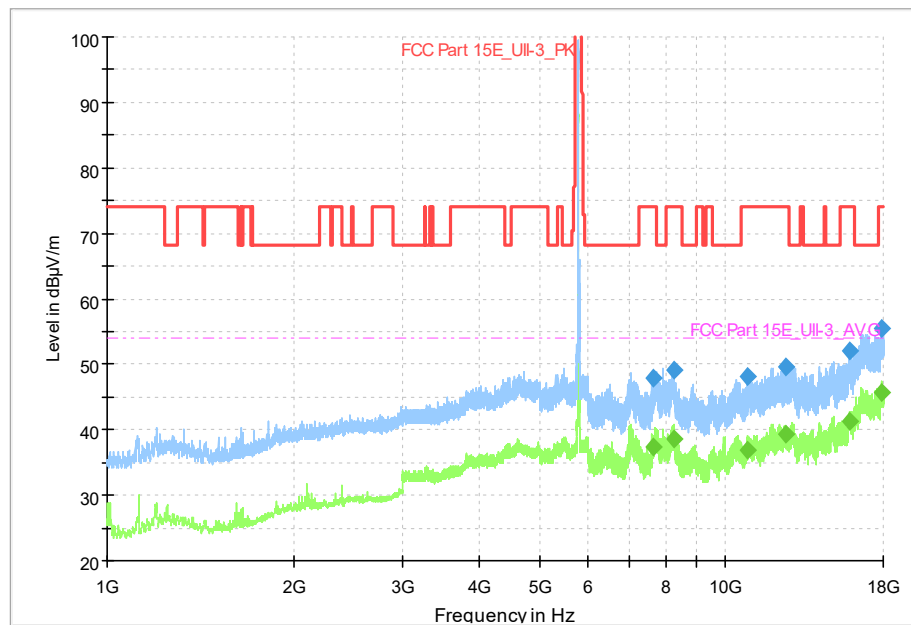
Fig. 67 Transmitter Spurious Emission (802.11ax-HE20, CH157 5785MHz, 1GHz-18GHz), MIMO
