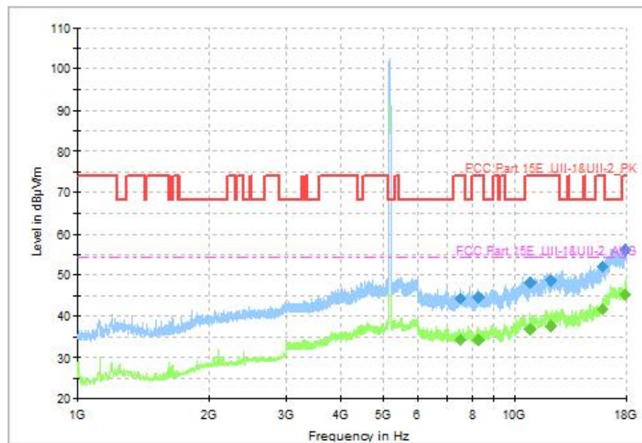
Fig. 69 Transmitter Spurious Emission (802.11n-HT40, CH38 5190MHz, 1GHz-18GHz), MIMO
