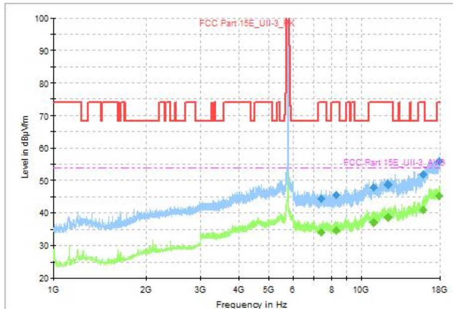
Fig. 74 Transmitter Spurious Emission (802.11ac-VHT80, CH155 5775MHz, 1GHz-18GHz), MIMO
