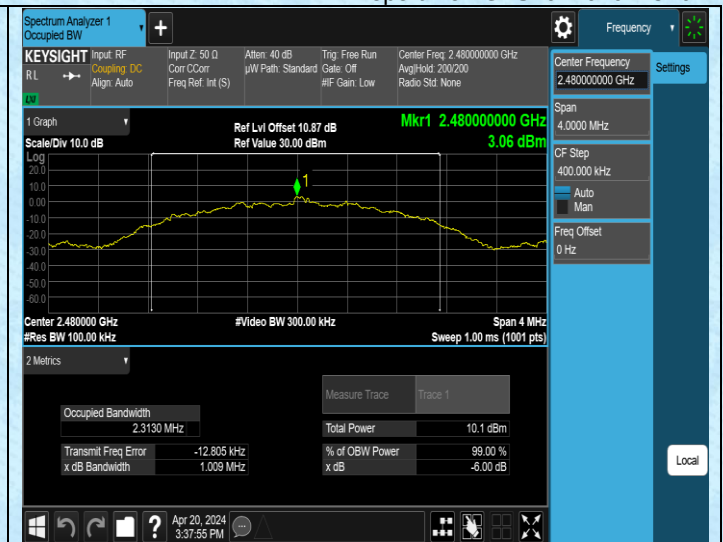
BLE_2M-Ant1-2480-PASS
