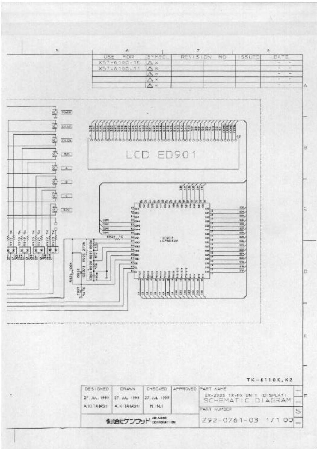
CIRCUIT SCHEMATIC(Display right)
