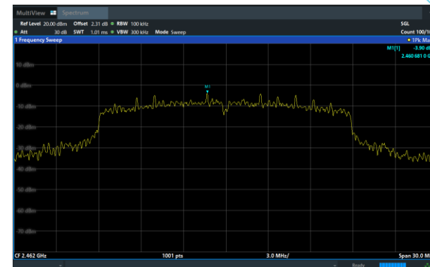
802.11n20: Band Edge, Right Side
