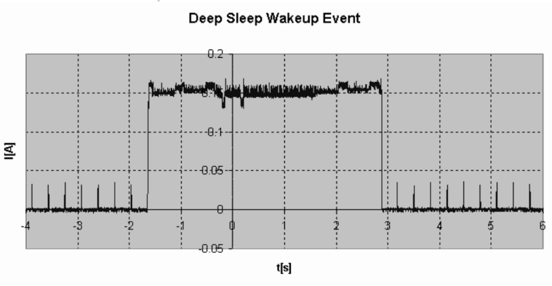
Figure 3-3: Current measurement for a wakeup event from deep sleep
