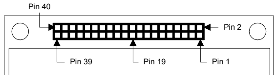
Figure 4-4: Pin 1 location (connector side)
