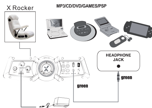
DIAGRAM 3 PORTABLE DEVICES
