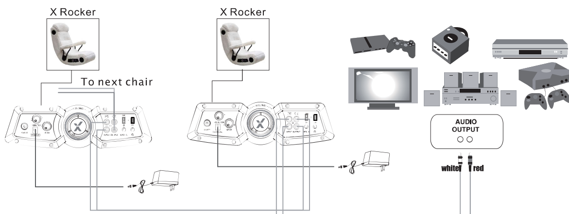
DIAGRAM 4 MULTI-USER CONNECTION
