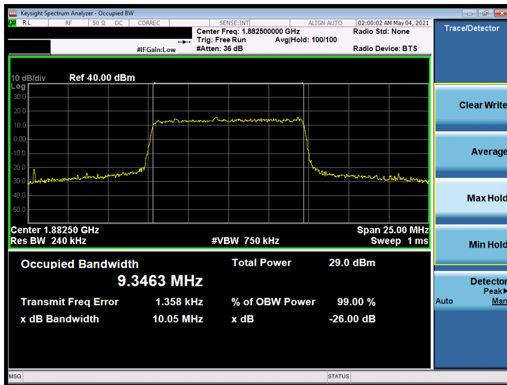
Plot 7-50. Occupied Bandwidth Plot (NR Band n25/2 - 10.0MHz CP-OFDM QPSK - Full RB)
