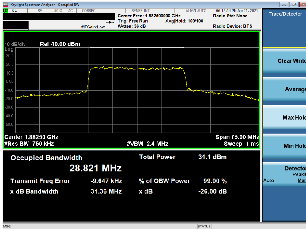
Plot 7-17. Occupied Bandwidth Plot (NR Band n25 - 30.0MHz CP-OFDM QPSK - Full RB)
