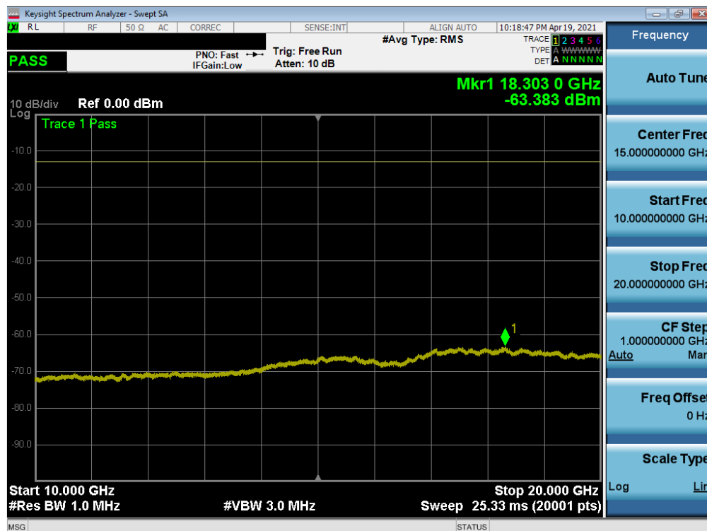
Plot 7-73. Conducted Spurious Plot (NR Band n25/2 - 20.0MHz - 1RB - Mid Channel)
