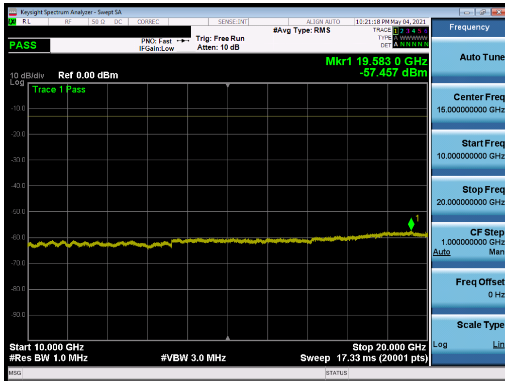
Plot 7-85. Conducted Spurious Plot (NR Band n25/2 - 20.0MHz - 1RB - High Channel)
