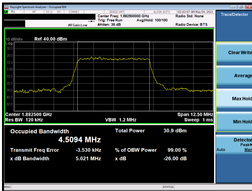
Plot 7-52. Occupied Bandwidth Plot (NR Band n25/2 - 5.0MHz DFT-s-OFDM BPSK - Full RB)
