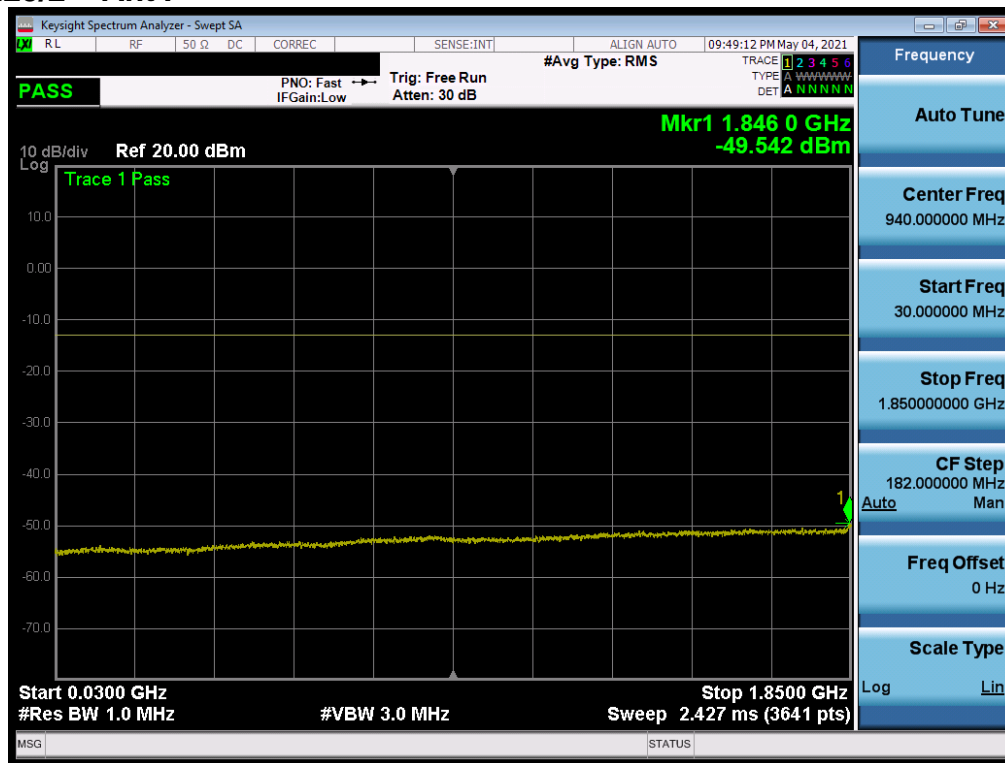
Plot 7-77. Conducted Spurious Plot (NR Band n25/2 -20.0MHz - 1RB - Low Channel)
