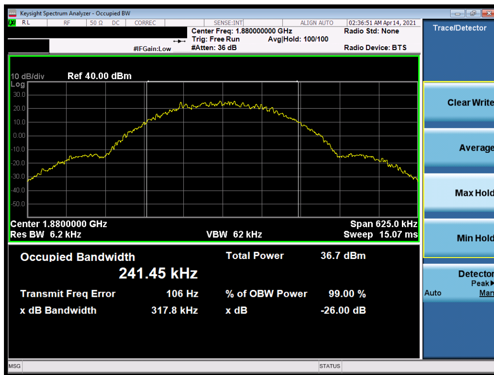
Plot 7-55. Occupied Bandwidth Plot (GPRS, Ch. 661)
