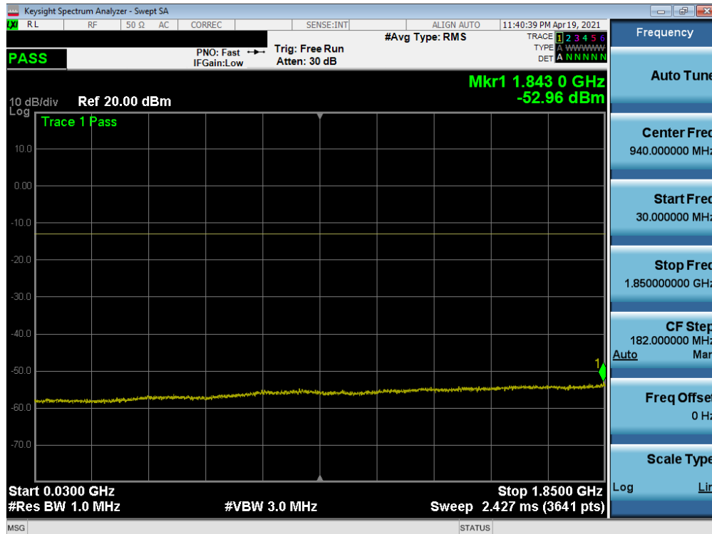
Plot 7-74. Conducted Spurious Plot (NR Band n25/2 - 20.0MHz - 1RB - High Channel)
