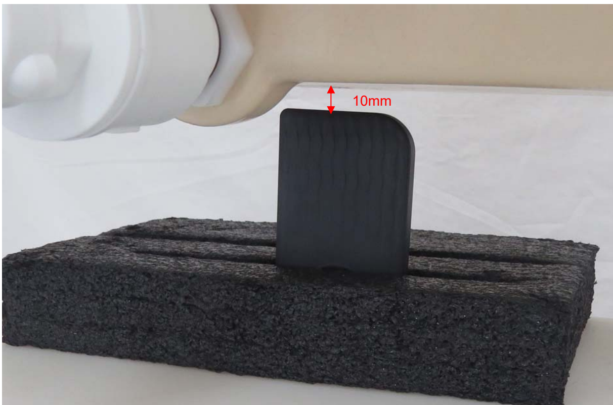
Picture 8: Bottom Edge, the distance from handset to the bottom of the Phantom is 10mm
