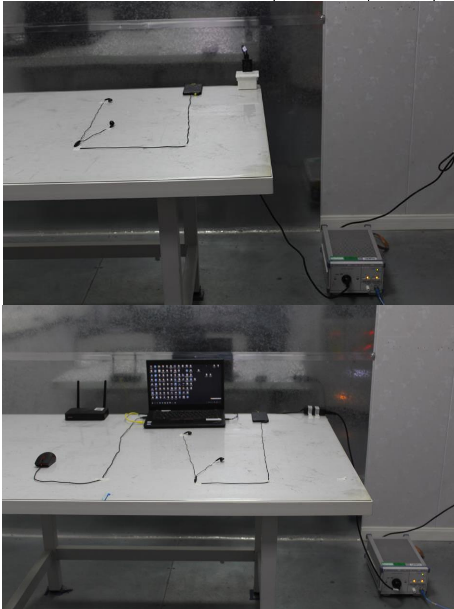
Conducted Emissions at Mains Terminals (150kHz-30MHz) Test Setup
