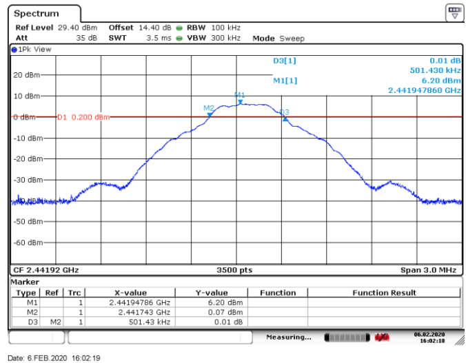
Figure 8.5-20: 6 dB bandwidth on mid channel, plot
