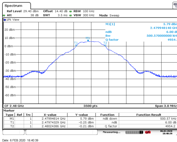
Figure 8.5-21: 6 dB bandwidth on high channel, plot
