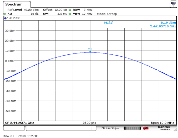
Figure 8.6-8: Output power on mid channel, 8DPSK Modulation
