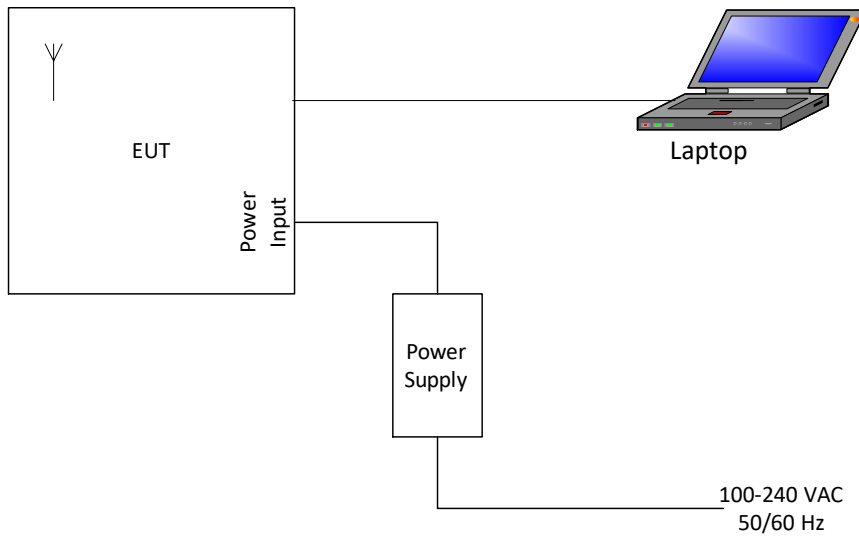
Figure 3.6-1: Setup diagram
