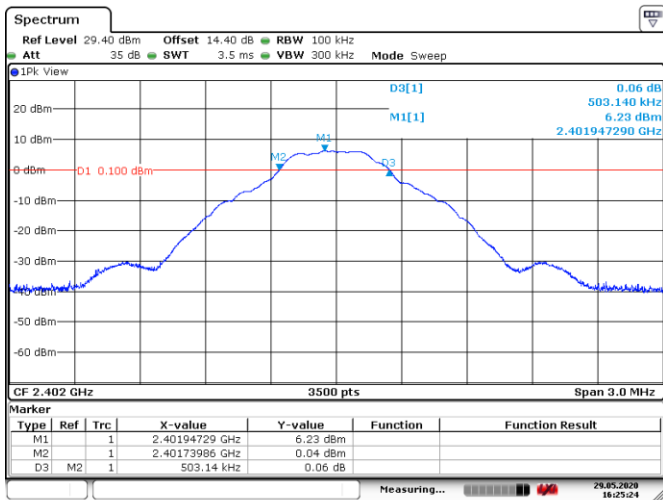
Figure 8.5-19: 6 dB bandwidth on low channel, plot
