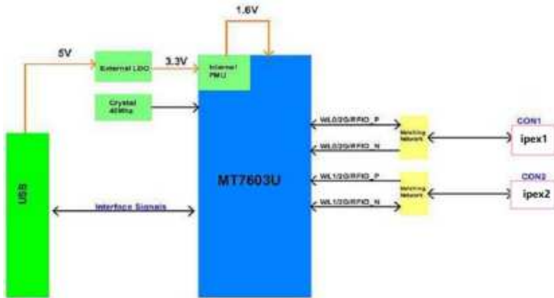
SKO.W603.6 Block Diagram
