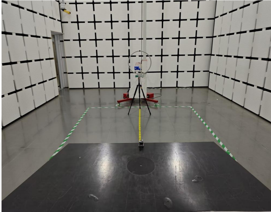
Spurious Radiation Emissions Test (9KHz-30MHz)
