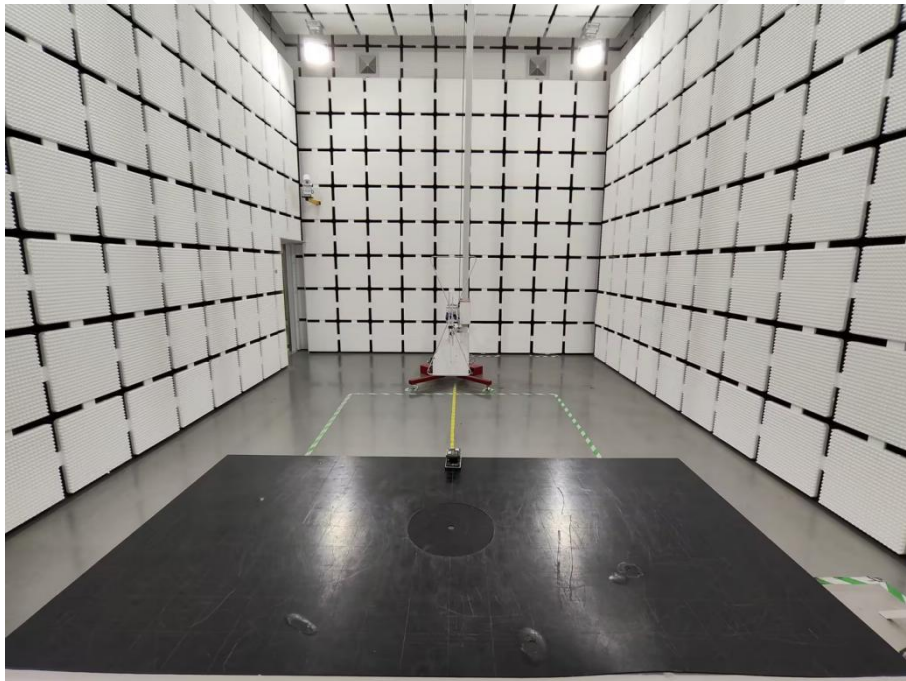
Spurious Radiation Emissions Test (30MHz-1G)
