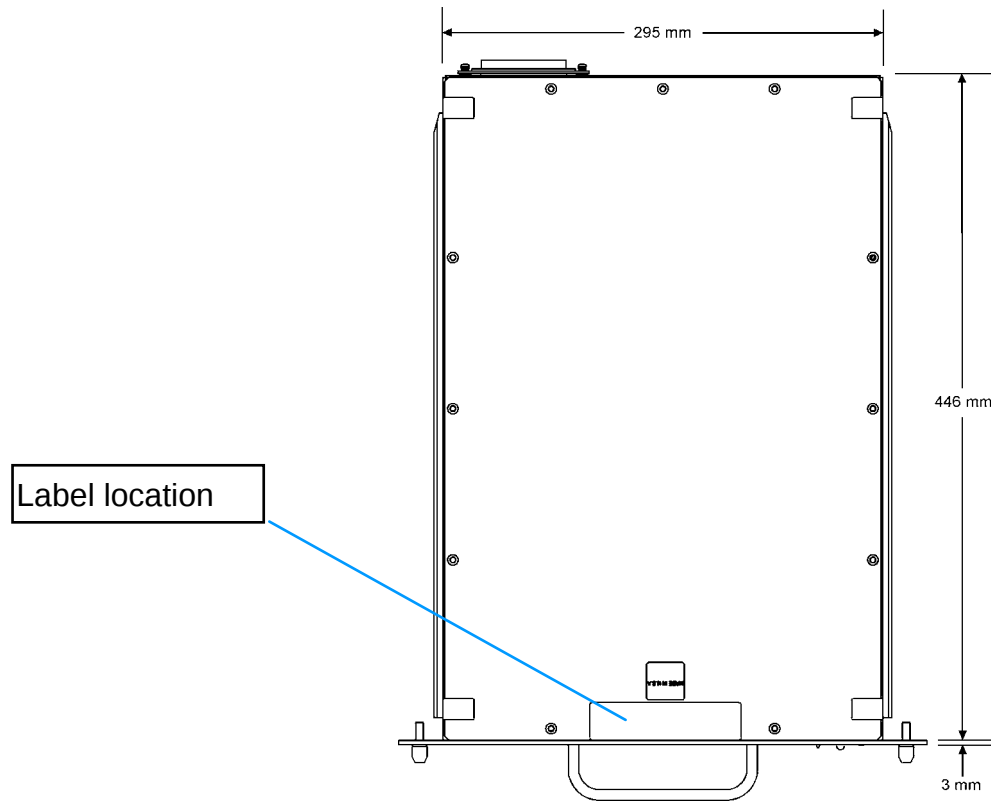
Figure 1-3 Model G3L-1929-120 Amplifier Top View
