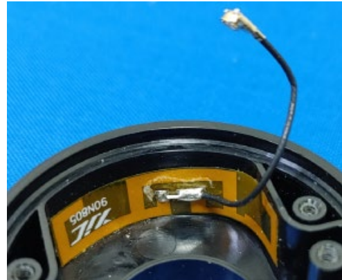
SRD Antenna
