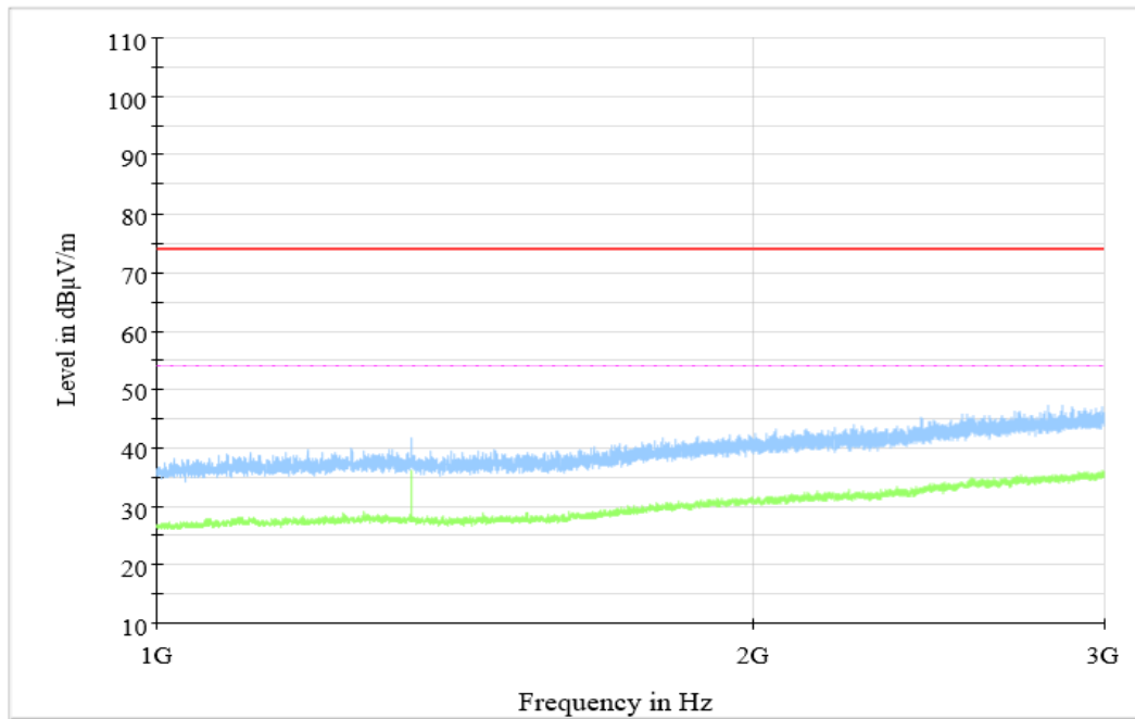
Figure A.1.32. Radiated Emission (Data Transfer : PC to TF Card,1GHz to 3GHz)
