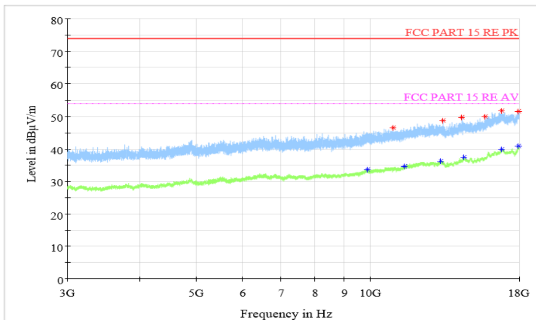
Figure A.1.39. Radiated Emission (Data Transfer : PC TO EUT, 3GHz to 18GHz)
