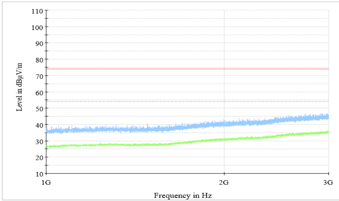
Figure A.1.23. Radiated Emission (FM receiver,1GHz to 3GHz)
