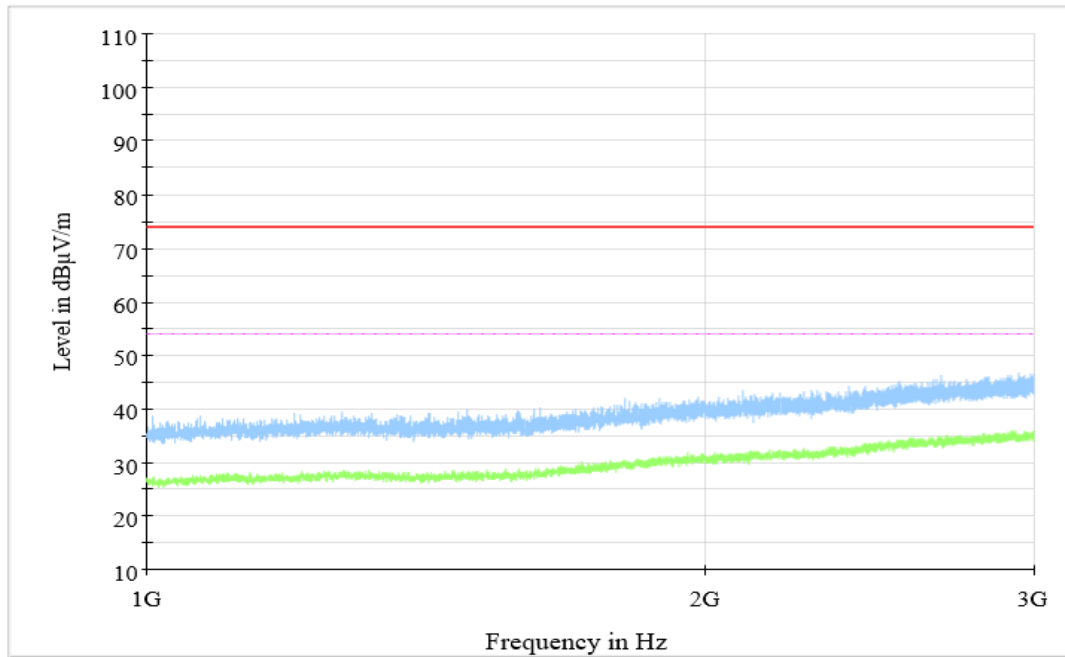
Figure A.1.14. Radiated Emission (FM receiver, 1GHz to 3GHz)
