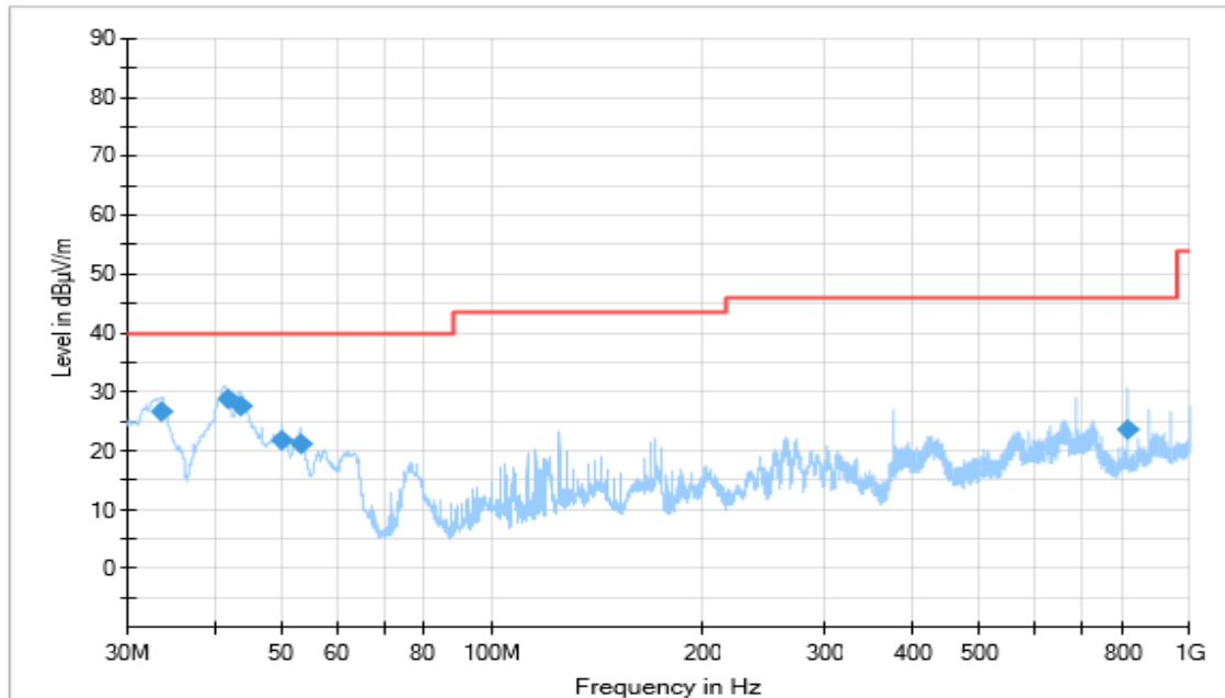
Fugure A.1.7. Radiated Emission (LTE Receiver Band 5, 30MHz to 1GHz)
