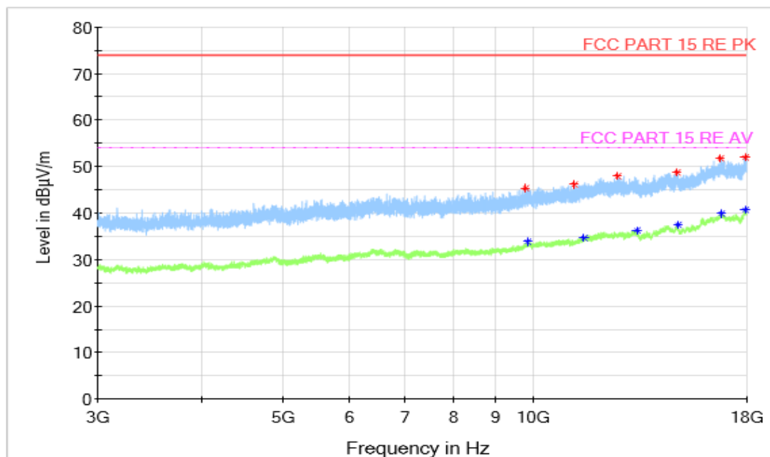
Figure A.1.12. Radiated Emission ( GSM Receiver 850MHz, 3GHz to 18GHz)
