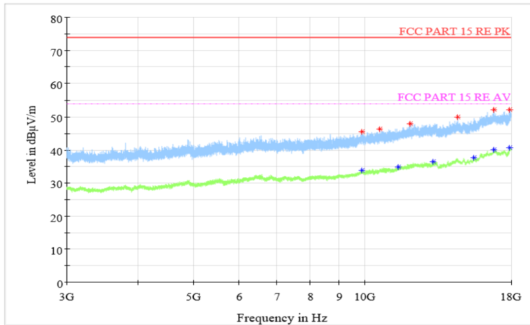
Figure A.1.30. Radiated Emission (Data Transfer : PC to EUT, 3GHz to 18GHz)
