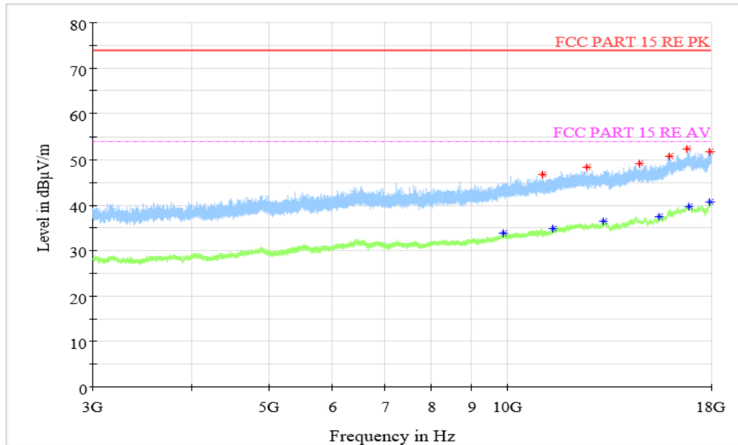
Figure A.1.36. Radiated Emission (Data Transfer : TF Card to PC, 3GHz to 18GHz)
