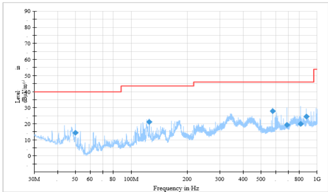
Figure A.1.31. Radiated Emission (Data Transfer : PC to TF Card, 30MHz to 1GHz)
