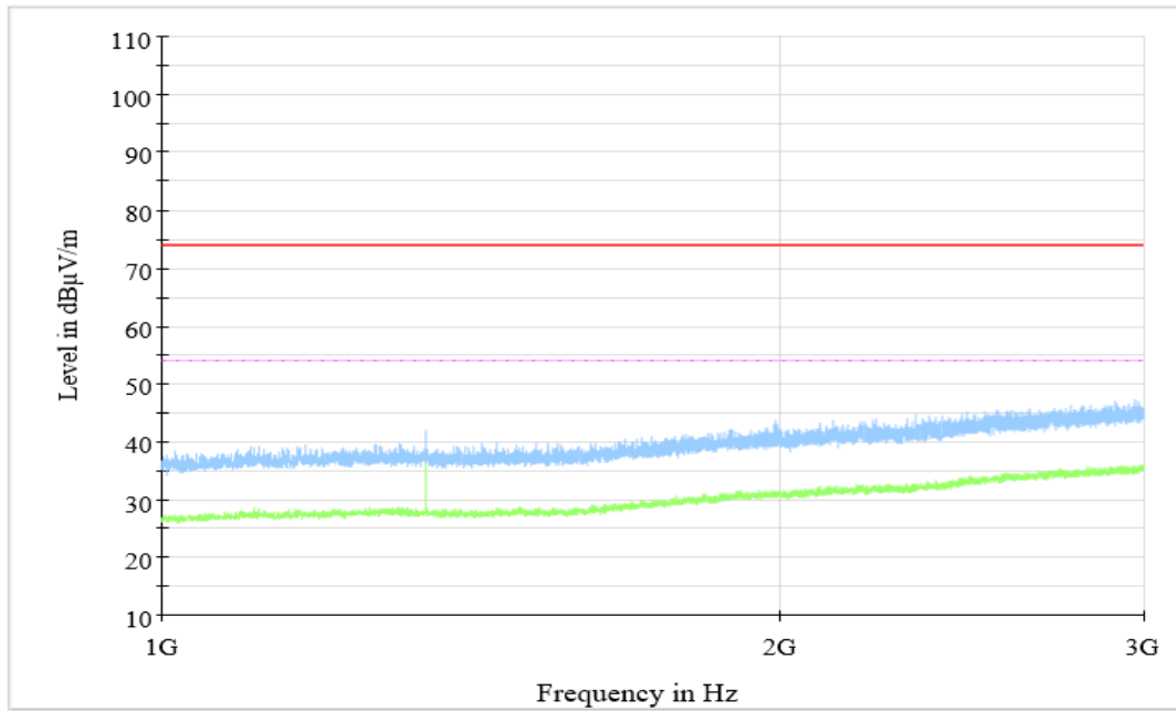
Figure A.1.38. Radiated Emission (Data Transfer : PC TO EUT,1GHz to 3GHz)
