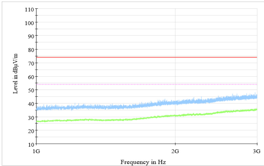
Figure A.1.26. Radiated Emission (Data Transfer : EUT to PC,1GHz to 3GHz)
