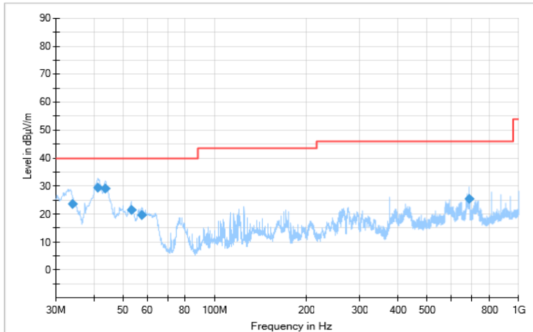
Figure A.1.4. Radiated Emission (WCDMA Receiver Band 5, 30MHz to 1GHz)
