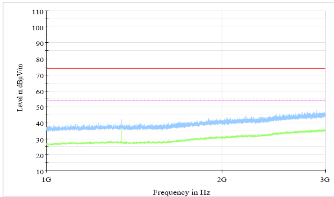
Figure A.1.35. Radiated Emission (Data Transfer : TF Card to PC,1GHz to 3GHz)
