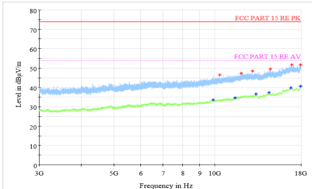
Figure A.1.33. Radiated Emission (Set.8, Data Transfer : PC to TF Card, 3GHz to 18GHz)
