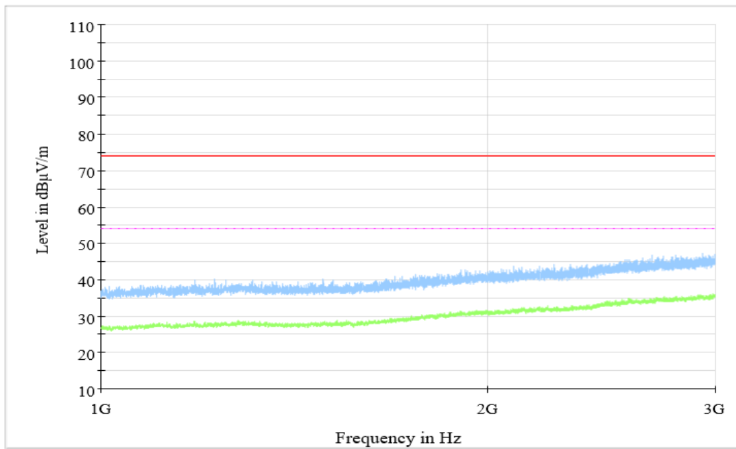
Figure A.1.29. Radiated Emission (Data Transfer : PC to EUT,1GHz to 3GHz)
