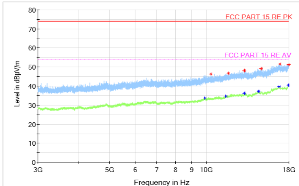
Figure A.1.6. Radiated Emission (WCDMA Receiver Band 5, 3GHz to 18GHz)
