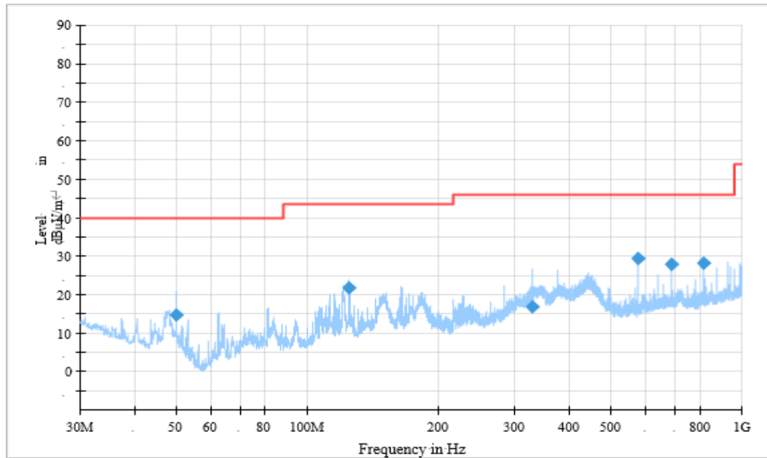
Figure A.1.34. Radiated Emission (Data Transfer : TF Card to PC, 30MHz to 1GHz)
