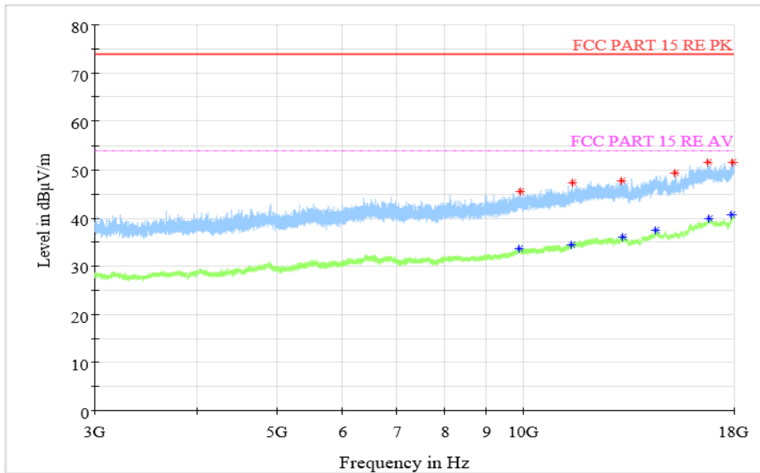
Figure A.1.18. Radiated Emission ( Video Player , 3GHz to 18GHz)
