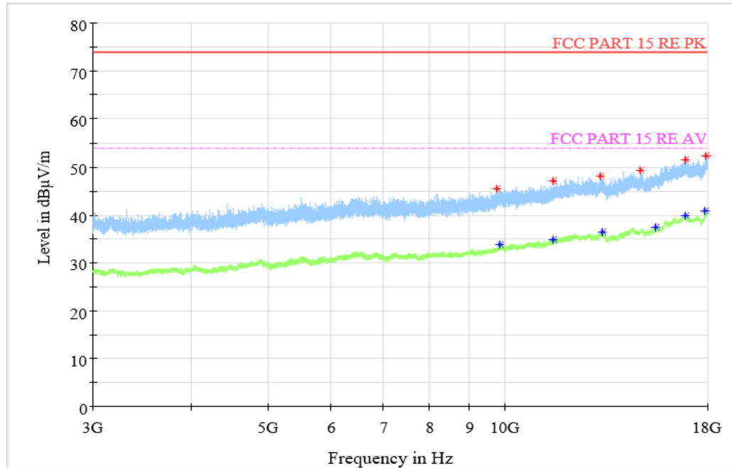
Figure A.1.27. Radiated Emission (Data Transfer : EUT to PC, 3GHz to 18GHz)
