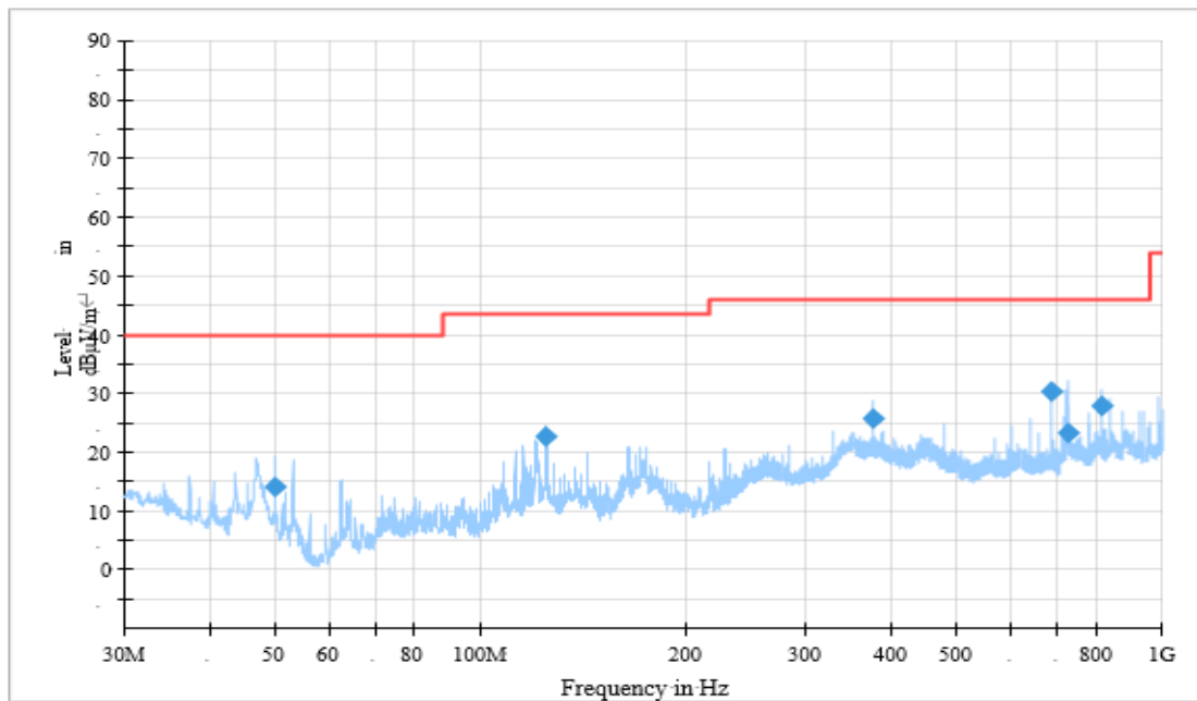
Figure A.1.28. Radiated Emission (Data Transfer : PC to EUT, 30MHz to 1GHz)
