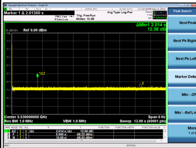
5530MHz - 12 sec (total 40001 bin, transmit data 1 bin[200ms~10s])
