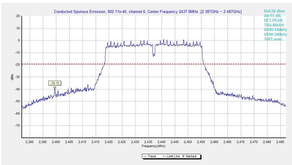
Fig.B.6.1.81 Transmitter Spurious Emission - Conducted (802.11n-HT40, Ch6, Center Frequency)
