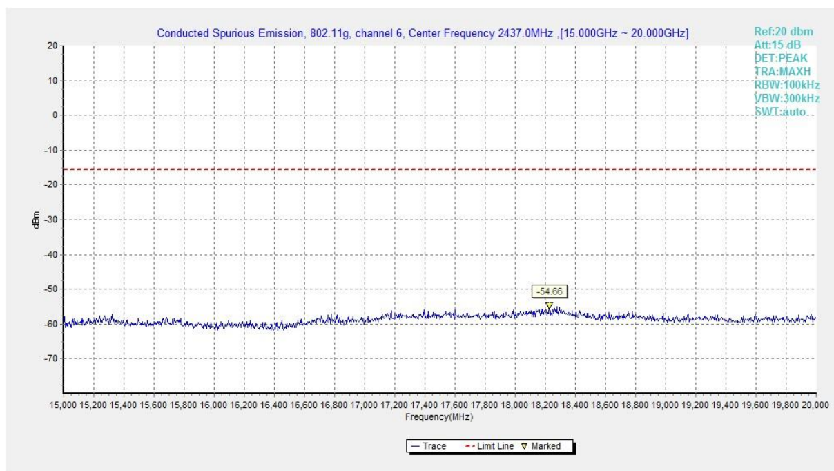
Fig.B.6.1.39 Transmitter Spurious Emission - Conducted (802.11g, Ch6, 15 GHz-20 GHz)
