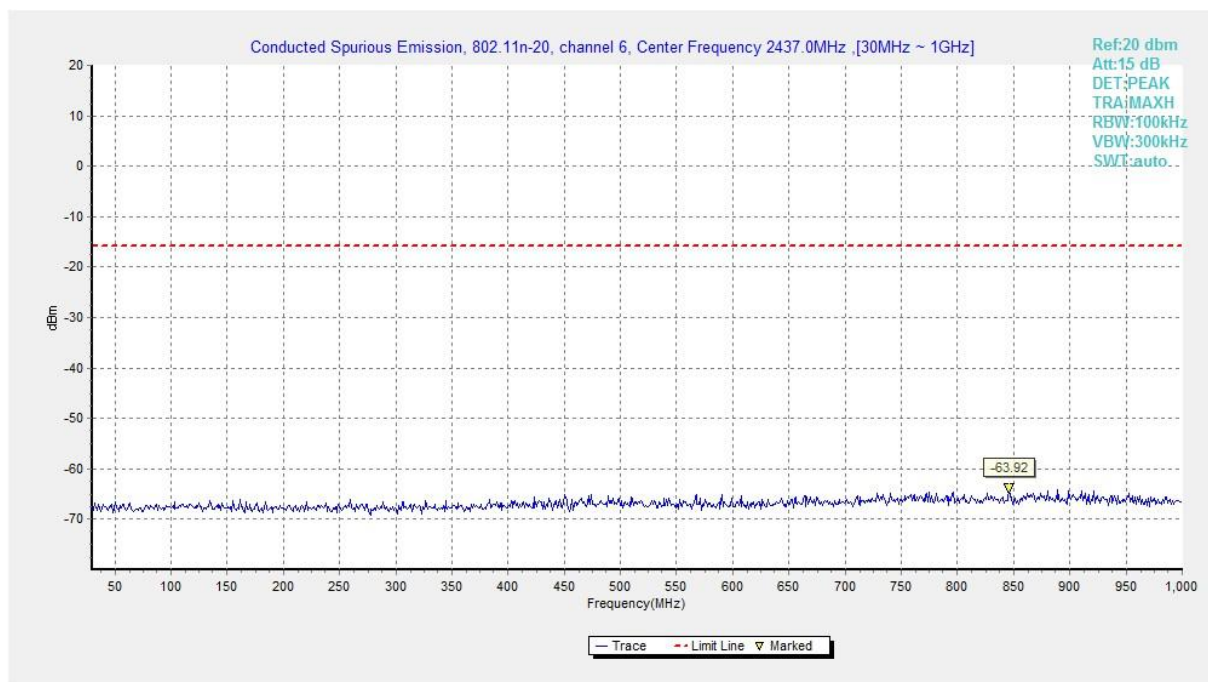
Fig.B.6.1.58 Transmitter Spurious Emission - Conducted (802.11n-HT20, Ch6, 30 MHz-1 GHz)
