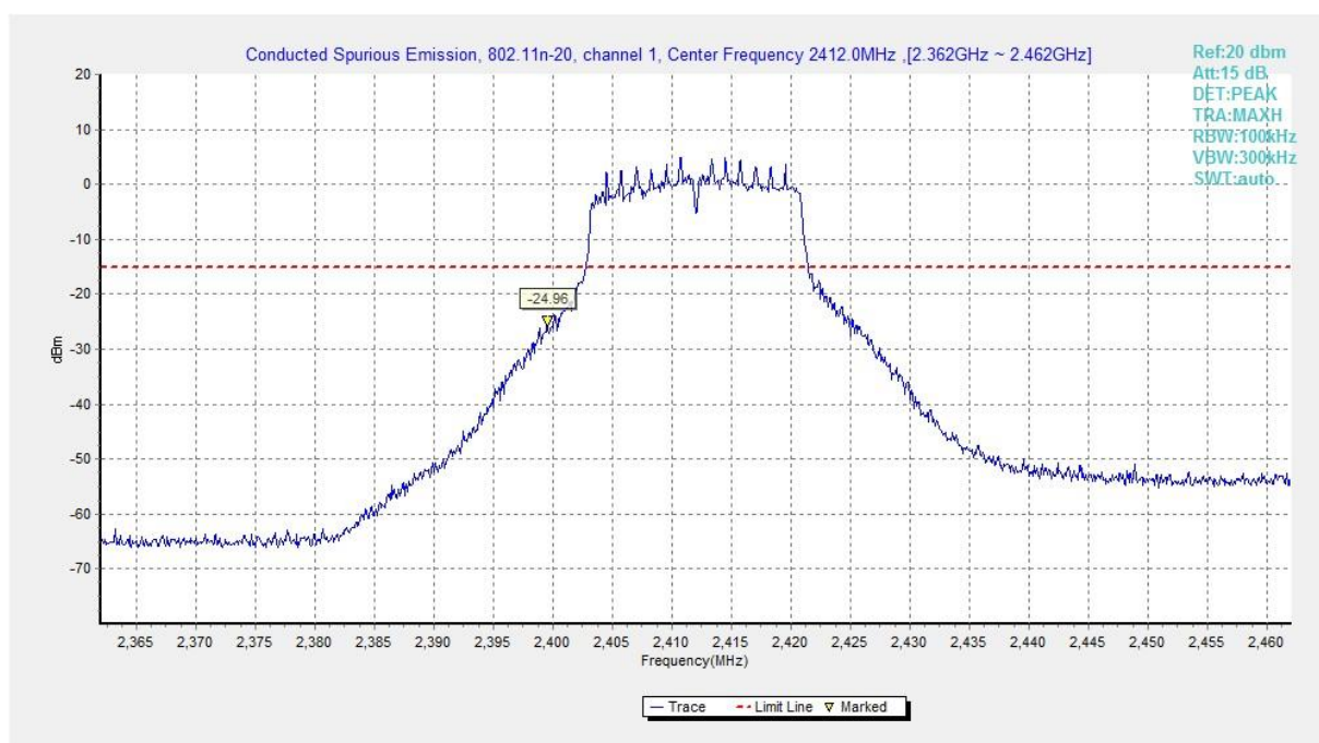
Fig.B.6.1.49 Transmitter Spurious Emission - Conducted (802.11n-HT20, Ch1, Center Frequency)
