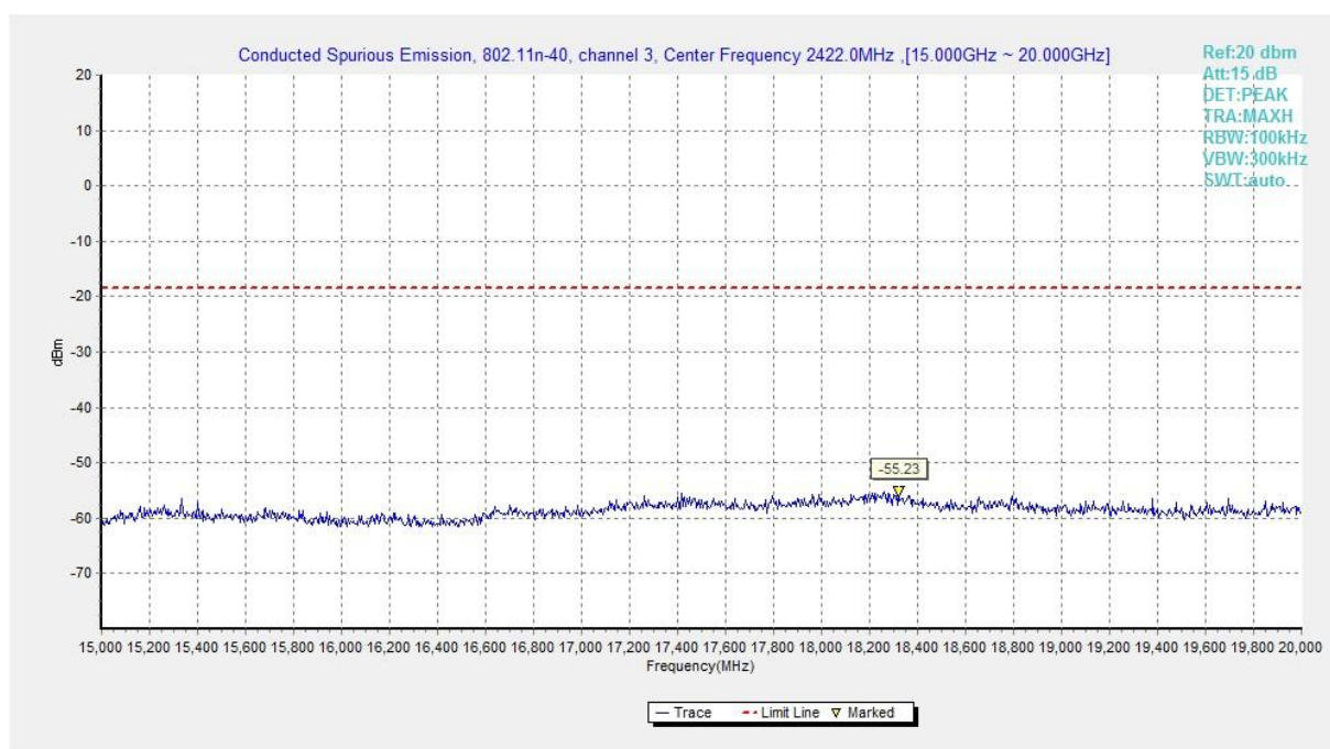
Fig.B.6.1.79 Transmitter Spurious Emission - Conducted (802.11n-HT40, Ch3, 15 GHz-20 GHz)
