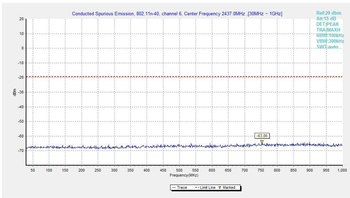
Fig.B.6.1.82 Transmitter Spurious Emission - Conducted (802.11n-HT40, Ch6, 30 MHz-1 GHz)
