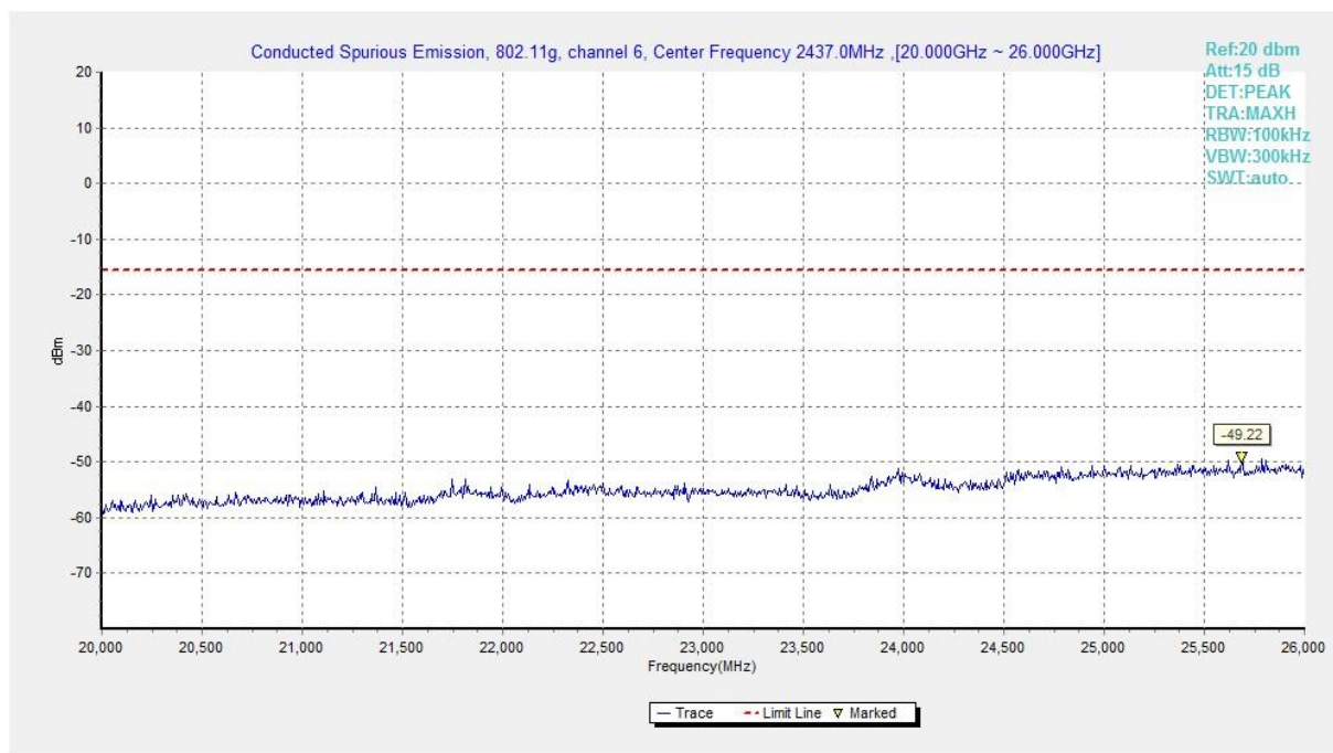
Fig.B.6.1.40 Transmitter Spurious Emission - Conducted (802.11g, Ch6, 20 GHz-26 GHz)
