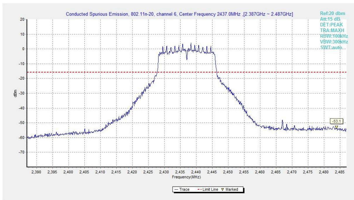
Fig.B.6.1.57 Transmitter Spurious Emission - Conducted (802.11n-HT20, Ch6, Center Frequency)
