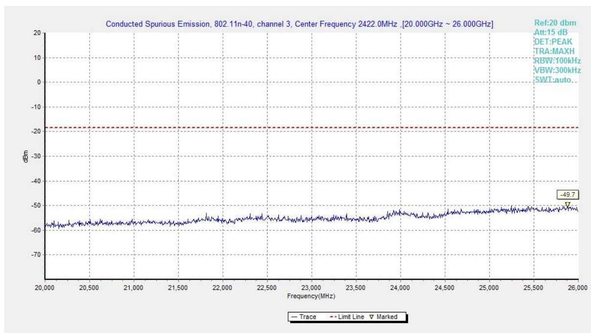
Fig.B.6.1.80 Transmitter Spurious Emission - Conducted (802.11n-HT40, Ch3, 20 GHz-26 GHz)
