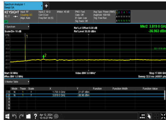
B5_N66(25M)_DFT-s- OFDM_QPSK_Edge_1RB_Left_Mid_CH
