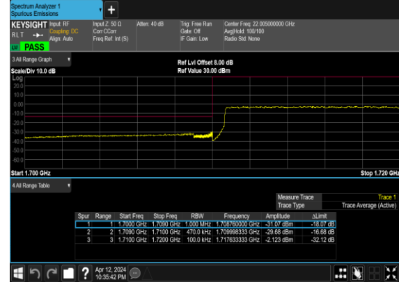
B5_N66(45M)_DFT-s- OFDM_BPSK_Outer_Full_Low_CH
