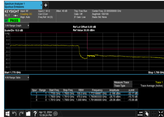
B5_N66(45M)_DFT-s- OFDM_BPSK_Outer_Full_High_CH
