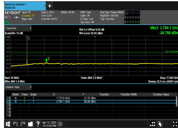
B5_N66(25M)_DFT-s- OFDM_QPSK_Edge_1RB_Left_Low_CH
