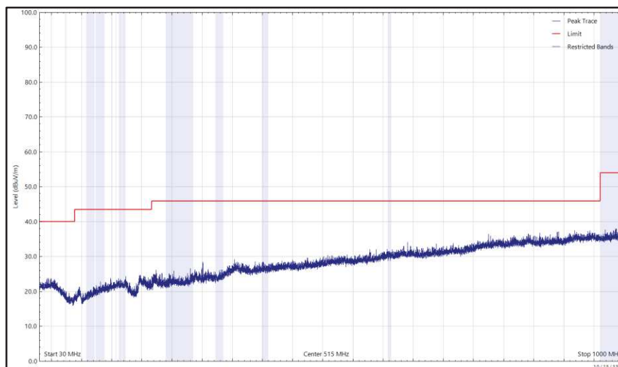
Figure 70 - 2440 MHz (CH18), Thread, iPA, Core 2 and U-NII-3 - 5785 MHz (CH157), VHT20, CDD, Core 0 + Core 1, 30 MHz to 1 GHz, Horizontal (Peak)
