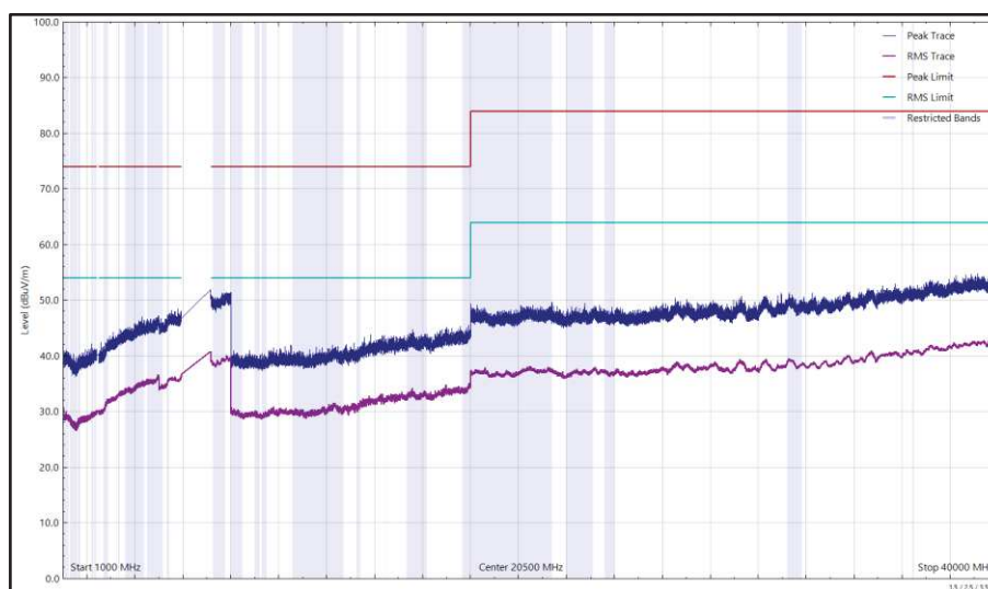
Figure 95 - 2440 MHz (CH18), Thread, iPA, Core 2 and U-NII-8 - 7115 MHz (CH233), HE20, SU, CDD, Core 0 + Core 1, 1 GHz to 40 GHz, Horizontal
