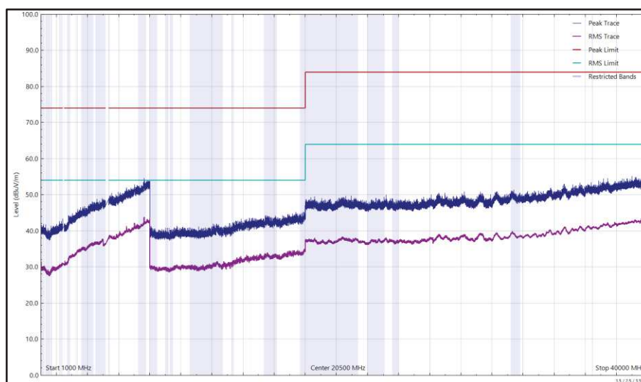
Figure 47 - 2440 MHz (CH18), Thread, iPA, Core 2 and U-NII-1 - 5240 MHz (CH48), VHT20, CDD, Core 0 + Core 1, 1 GHz to 40 GHz, Horizontal
