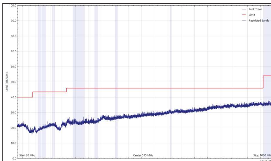
Figure 94 - 2440 MHz (CH18), Thread, iPA, Core 2 and U-NII-8 - 7115 MHz (CH233), HE20, SU, CDD, Core 0 + Core 1, 30 MHz to 1 GHz, Horizontal (Peak)
