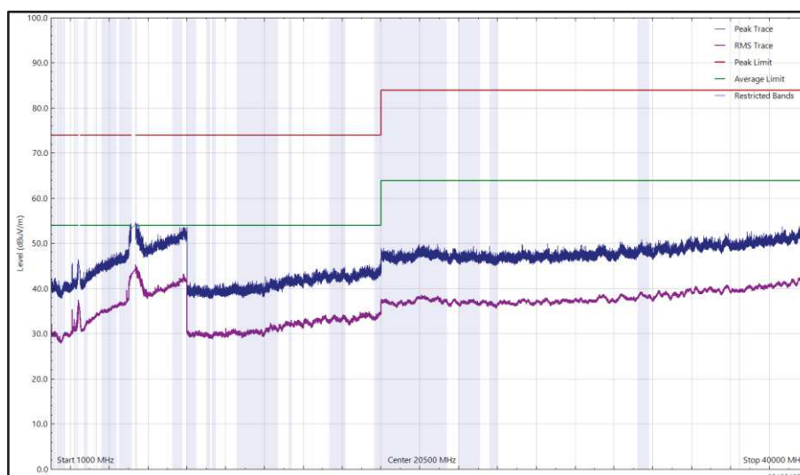
Figure 11 - 2441 MHz (CH39), DH5, ePA, Core 0 + Core 1 and U-NII-1 - 5240 MHz (CH48), VHT20, CDD, Core 0 + Core 1, 1 GHz to 40 GHz, Horizontal
