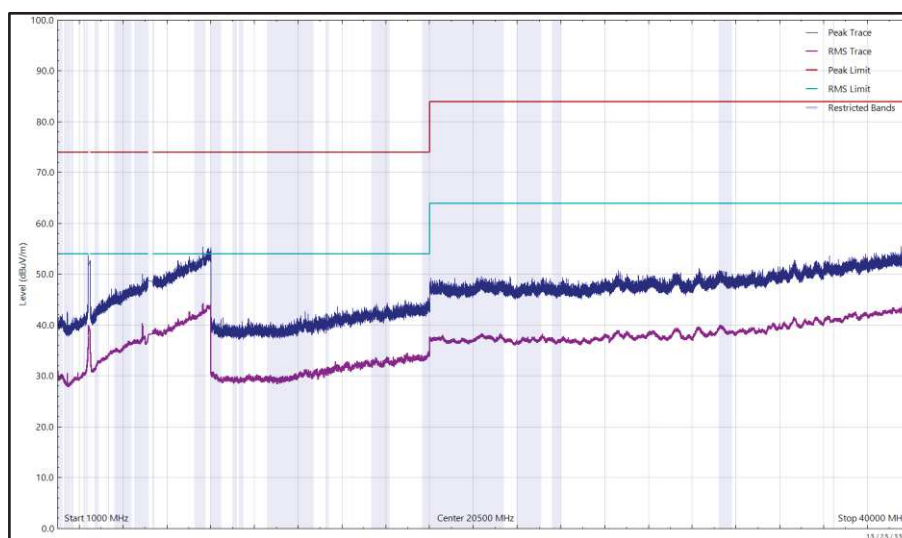
Figure 31 - 2437 MHz (CH6), HT20, Core 1 and 5204 MHz, HDR8, ePA, Core 0, 1 GHz to 40 GHz, Horizontal
