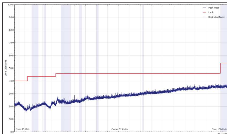
Figure 46 - 2440 MHz (CH18), Thread, iPA, Core 2 and U-NII-1 - 5240 MHz (CH48), VHT20, CDD, Core 0 + Core 1, 30 MHz to 1 GHz, Horizontal (Peak)
