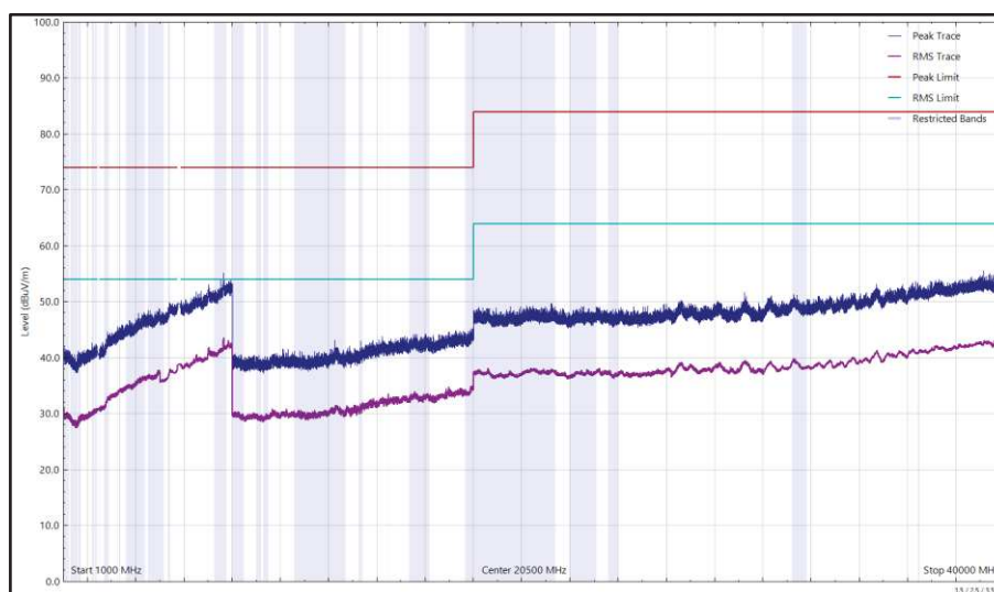
Figure 71 - 2440 MHz (CH18), Thread, iPA, Core 2 and U-NII-3 - 5785 MHz (CH157), VHT20, CDD, Core 0 + Core 1, 1 GHz to 40 GHz, Horizontal
