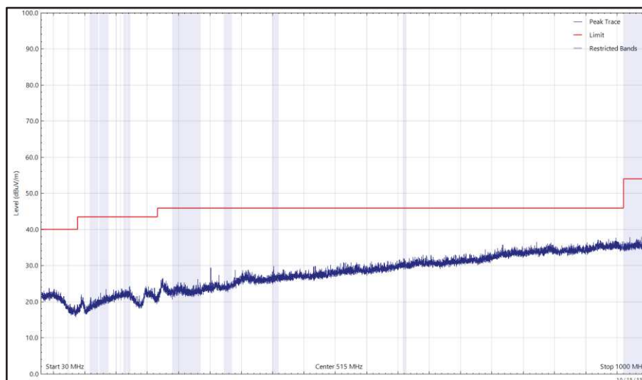
Figure 42 - 2440 MHz (CH18), Thread, ePA, Core 1 and U-NII-1 - 5240 MHz (CH48), VHT20, CDD, Core 0 + Core 1, 30 MHz to 1 GHz, Horizontal (Peak)
