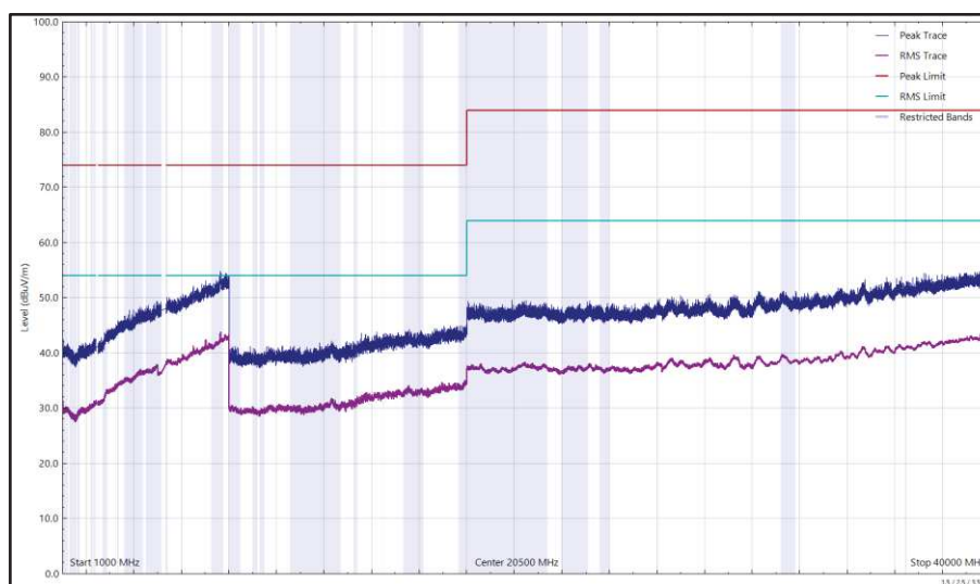
Figure 43 - 2440 MHz (CH18), Thread, ePA, Core 1 and U-NII-1 - 5240 MHz (CH48), VHT20, CDD, Core 0 + Core 1, 1 GHz to 40 GHz, Horizontal
