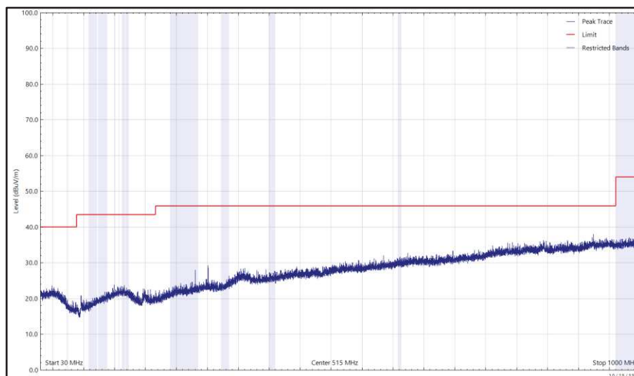
Figure 30 - 2437 MHz (CH6), HT20, Core 1 and 5204 MHz, HDR8, ePA, Core 0, 30 MHz to 1 GHz, Horizontal (Peak)
