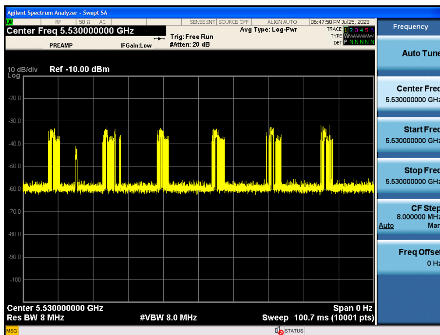
Channel Loading Plot - 802.11ax80-5530MHz
