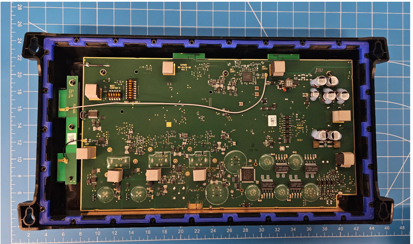
Unit Back- Lid Removed
