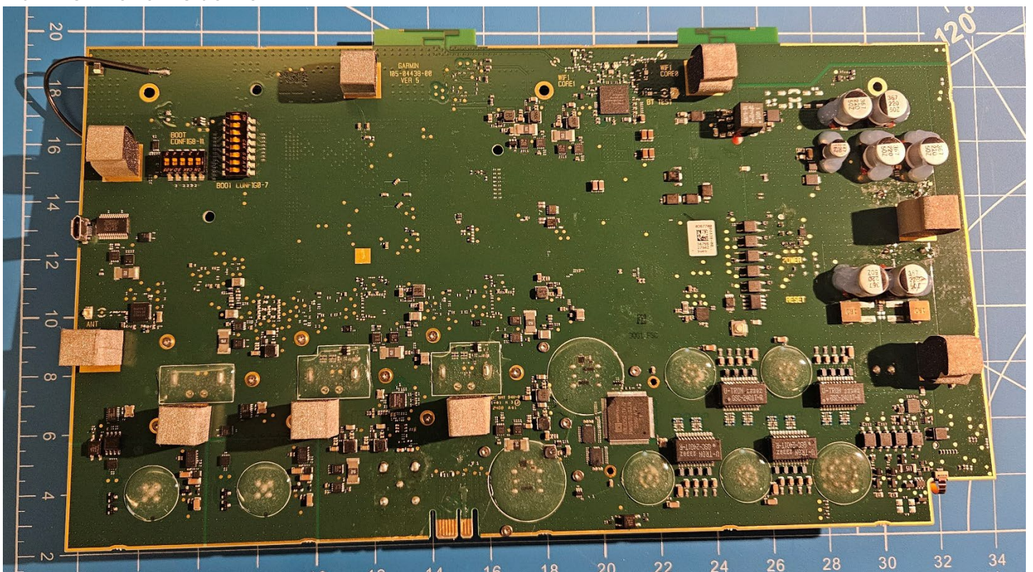
Main PCB Bottom Side View
