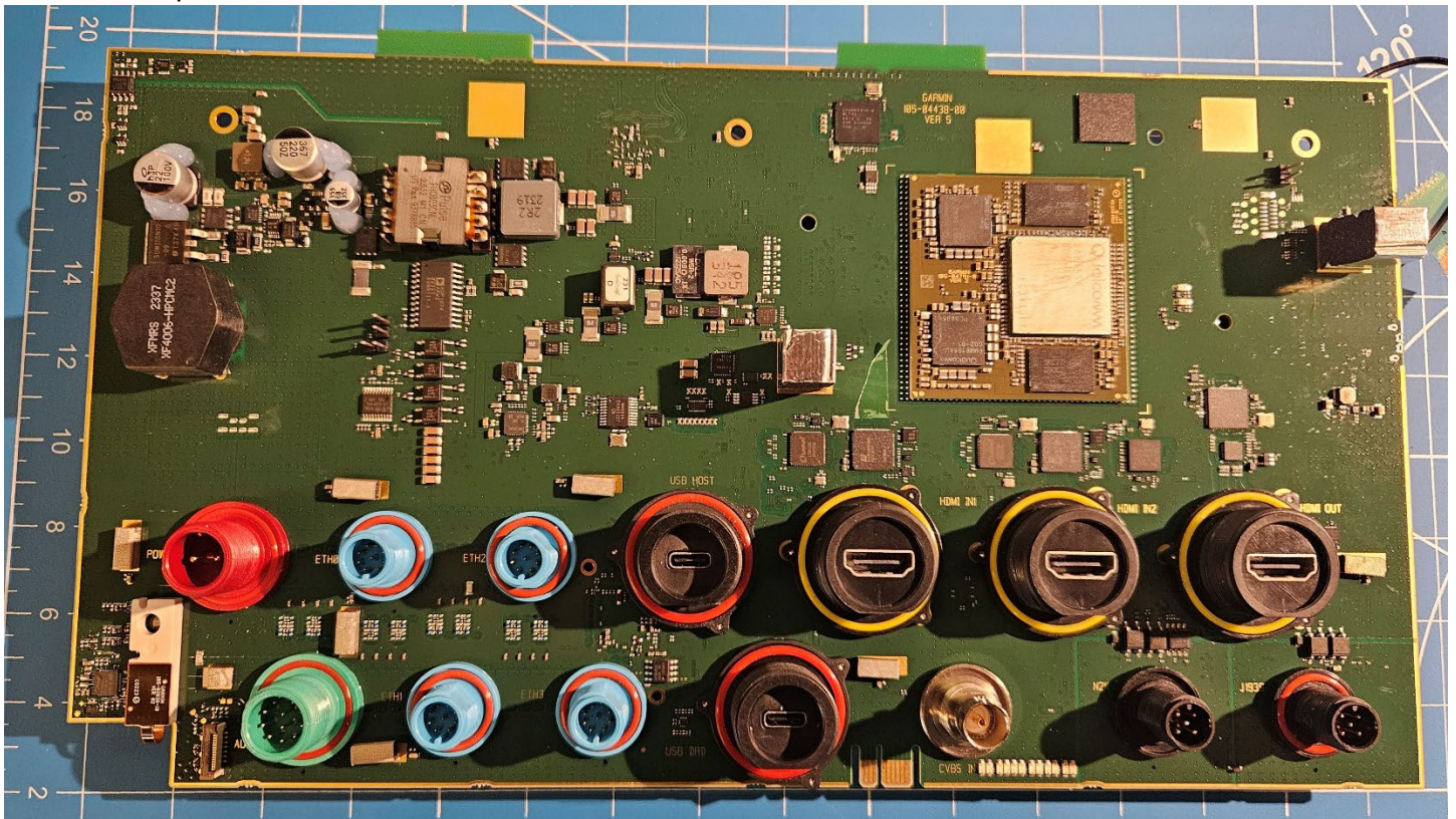
Main PCB Top Side
