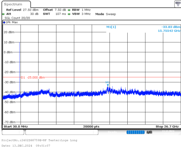
10MHz_Low_QPSK_1@0(30MHz~26.7GHz)
