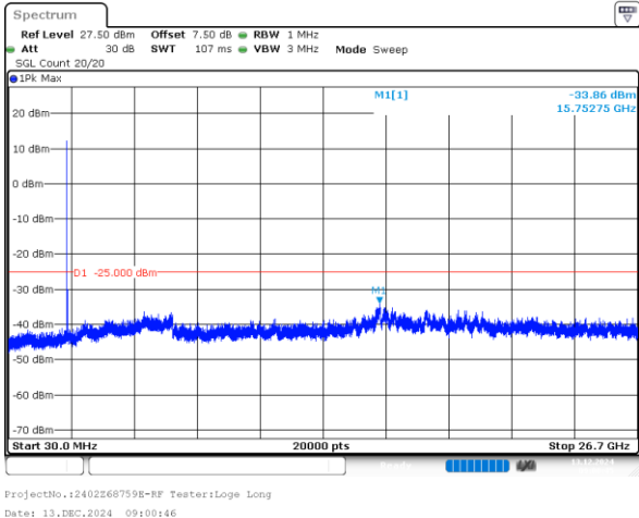
5MHz_High_QPSK_1@0(30MHz~26.7GHz)
