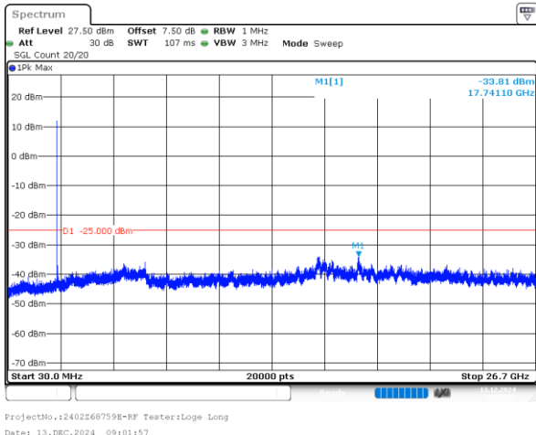
10MHz_High_QPSK_1@0(30MHz~26.7GHz)
