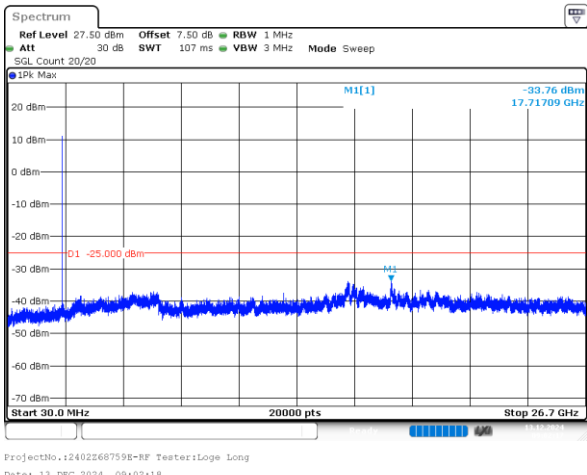
10MHz_Middle_QPSK_1@0(30MHz~26.7GHz)
