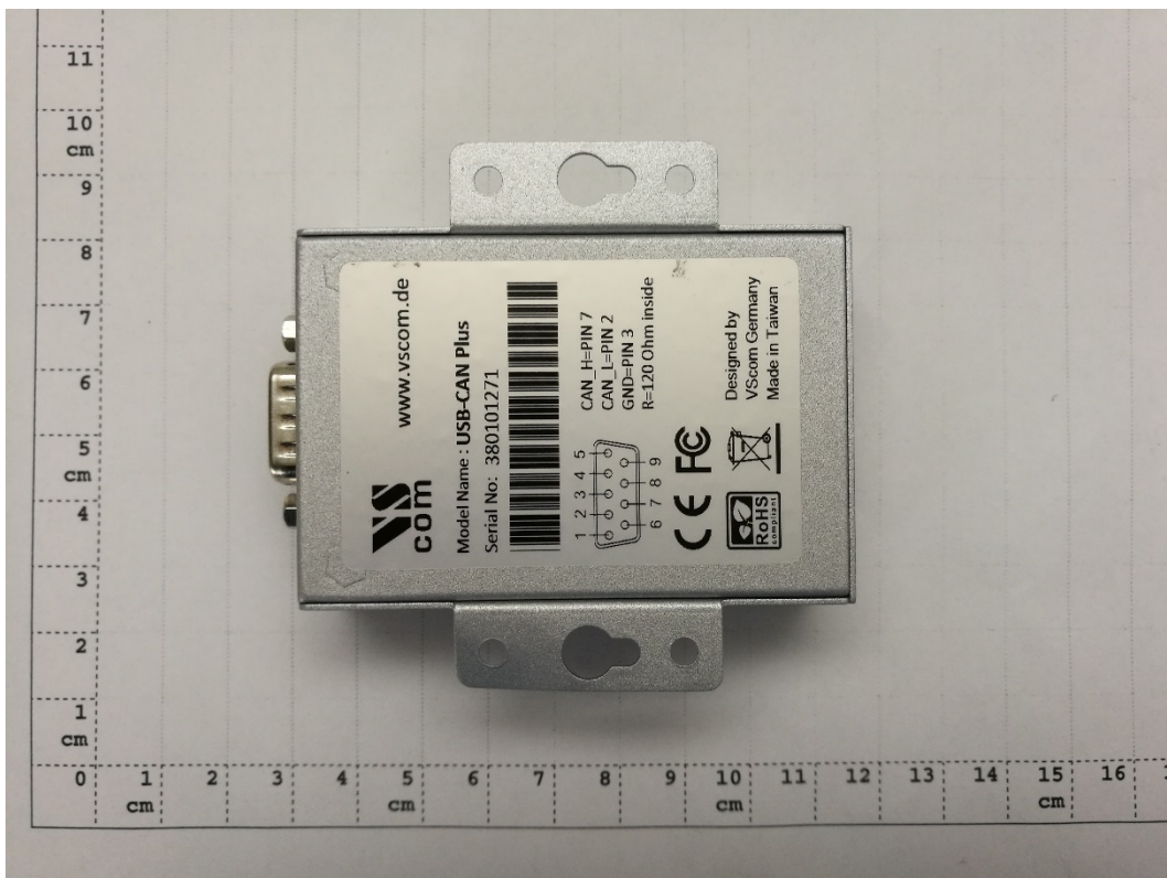
Diagram 6: AE 1 (VScom USB-CAN Adapter) back side
