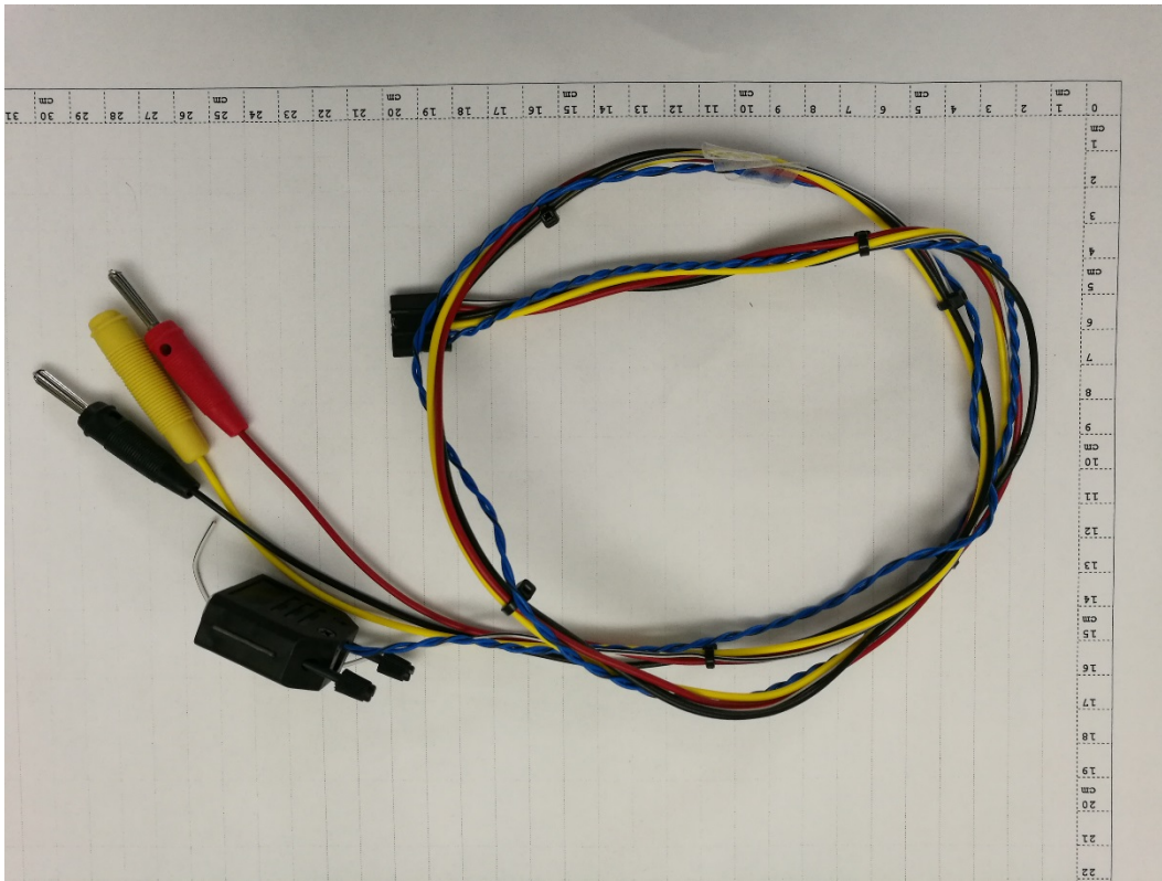
Diagram 9: Main harness
