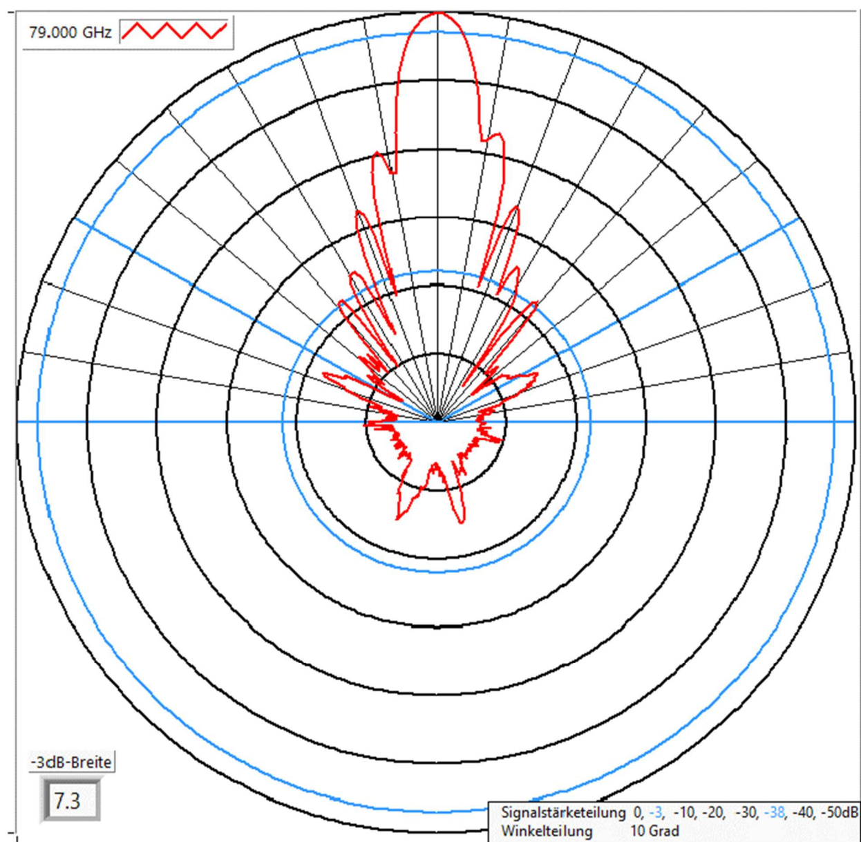
Antenna diagram as provided by the applicant in the E-plane
