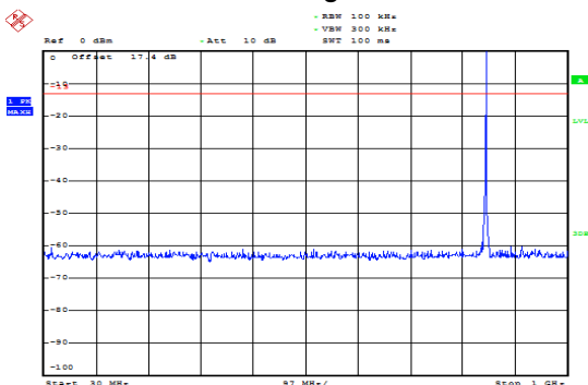
GSM 850 CH-High 30MHz ~ 1GHz
