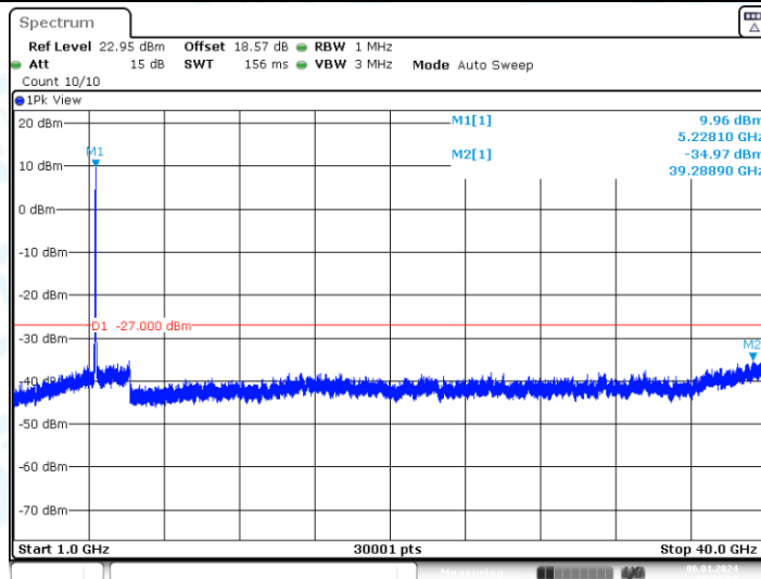
11AC40-CDD_Ant2_5230_1000~40000
