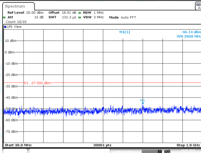
11AX20-CDD_Ant2_5700_30~1000
