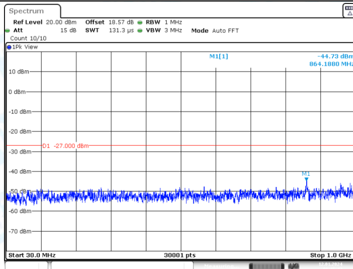
11AX20-CDD_Ant2_5240_30~1000
