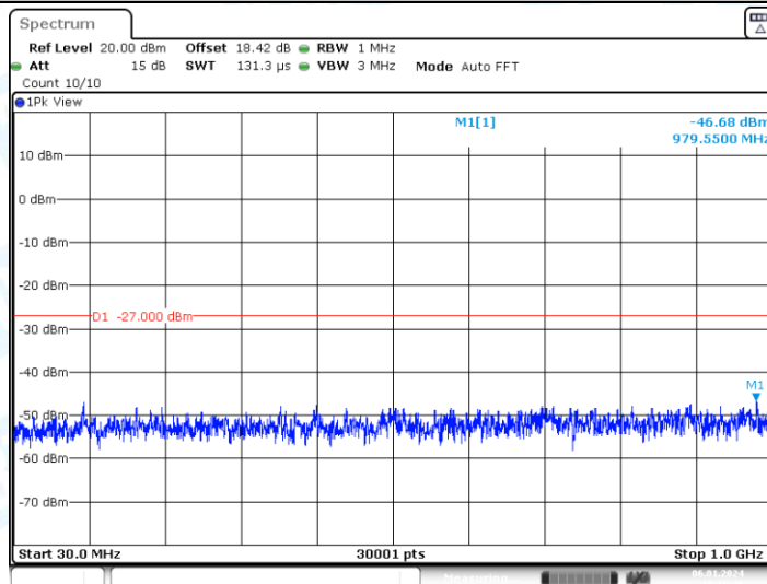
11AC40-CDD_Ant1_5270_30~1000
