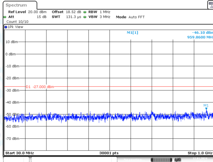
11AX20-CDD_Ant2_5320_30~1000
