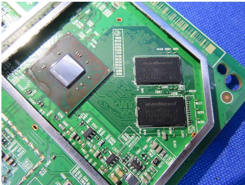
(10) EUT Photo (Model No.: u4m GM1028, u4m-2 GM1028-2)
