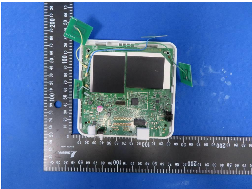
(2) EUT Photo (Model No.: u4m GM1028, u4m-2 GM1028-2)
