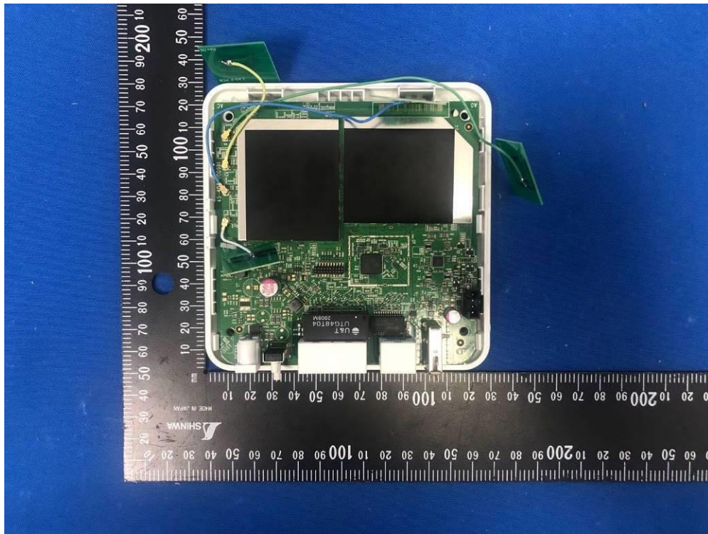
(15) EUT Photo (Model No.: u4 GS2028E, u4-2 GS2028E-2)
