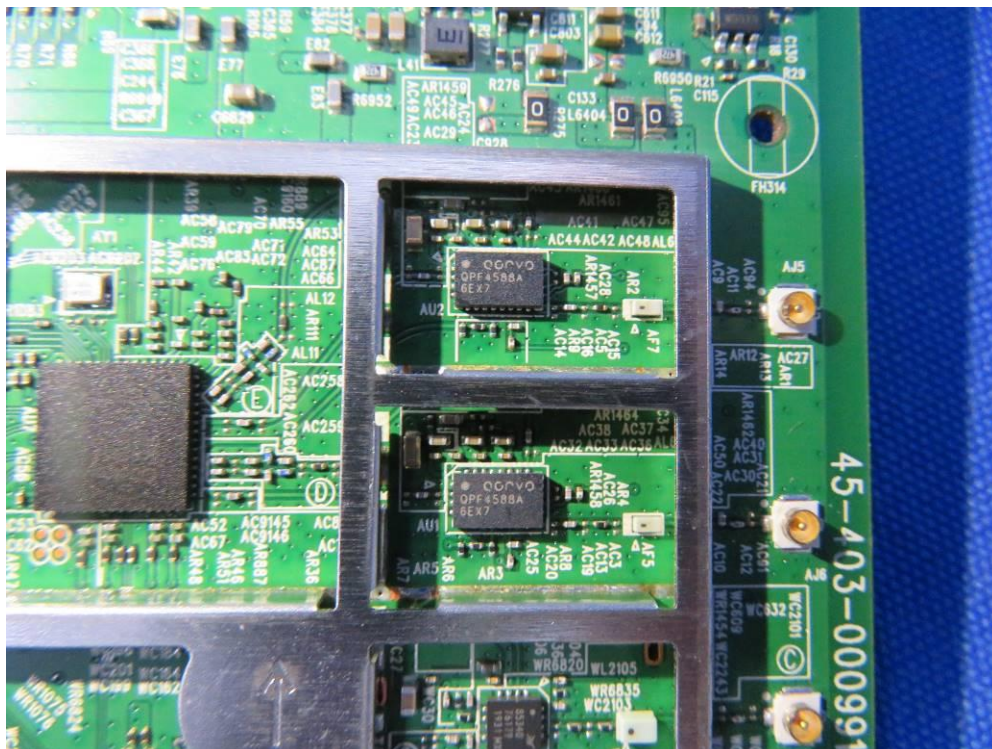
(12) EUT Photo (Model No.: u4m GM1028, u4m-2 GM1028-2)
