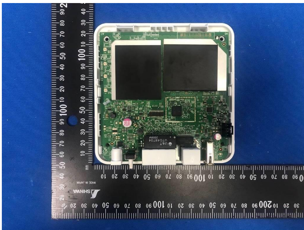
(16) EUT Photo (Model No.: u4 GS2028E, u4-2 GS2028E-2)
