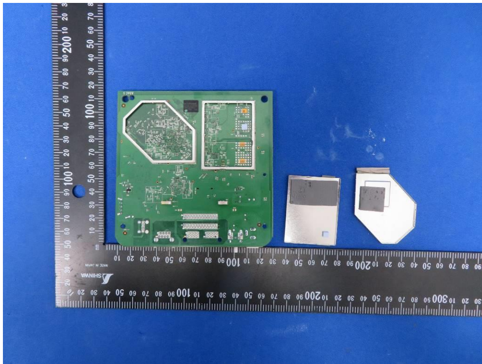
(5) EUT Photo (Model No.: u4m GM1028, u4m-2 GM1028-2)
