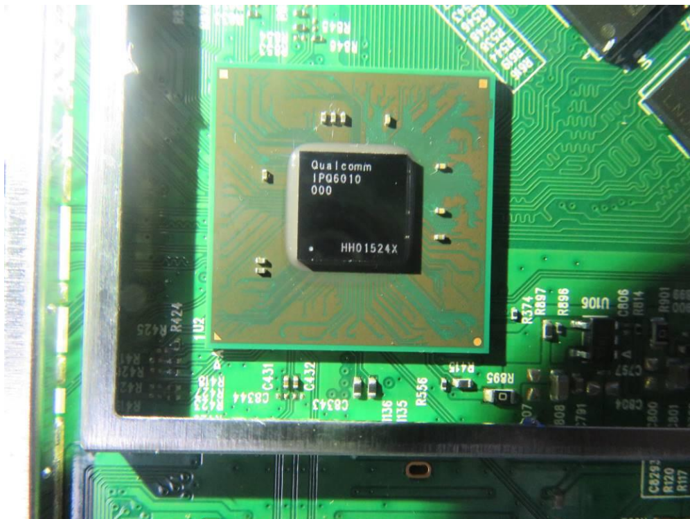
(22) EUT Photo (Model No.: u4 GS2028E, u4-2 GS2028E-2)
