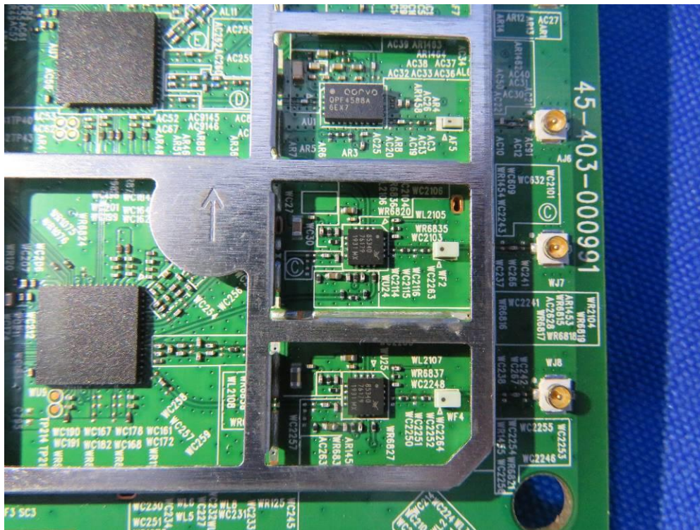
(13) EUT Photo (Model No.: u4m GM1028, u4m-2 GM1028-2)
