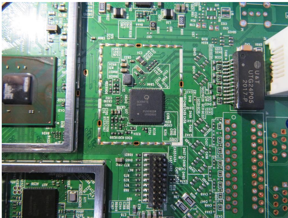
(8) EUT Photo (Model No.: u4m GM1028, u4m-2 GM1028-2)
