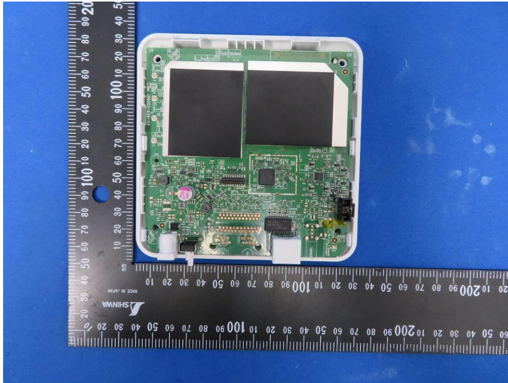
(3) EUT Photo (Model No.: u4m GM1028, u4m-2 GM1028-2)
