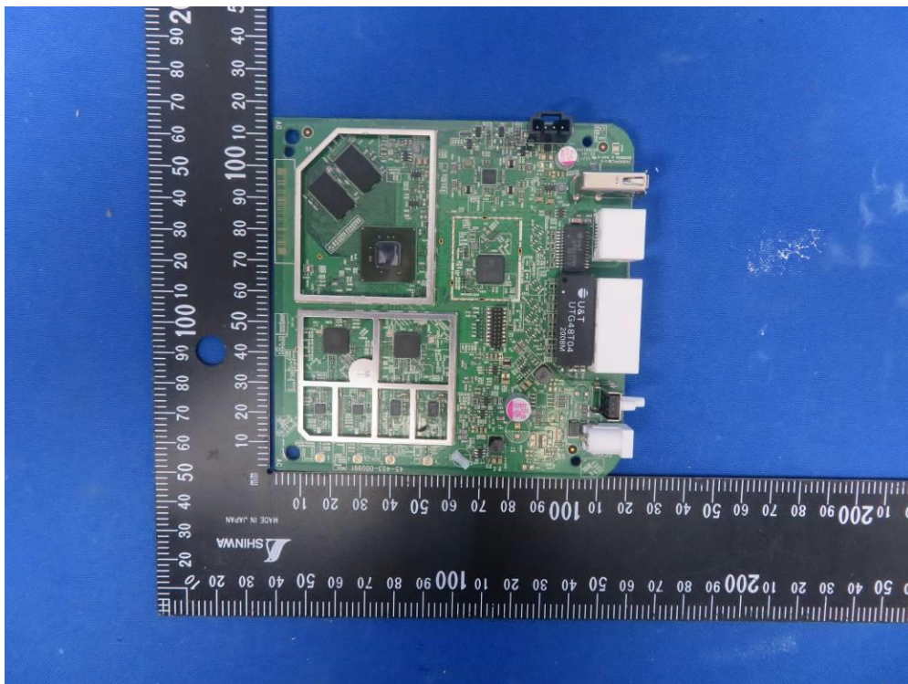
(20) EUT Photo (Model No.: u4 GS2028E, u4-2 GS2028E-2)
