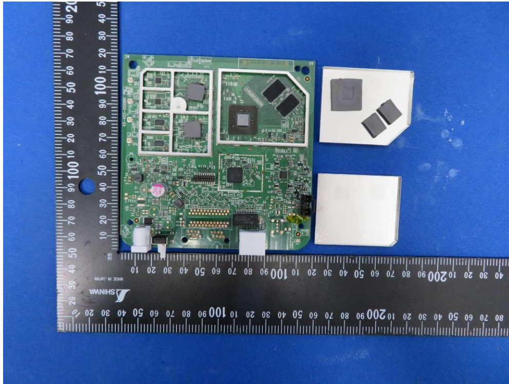
(7) EUT Photo (Model No.: u4m GM1028, u4m-2 GM1028-2)
