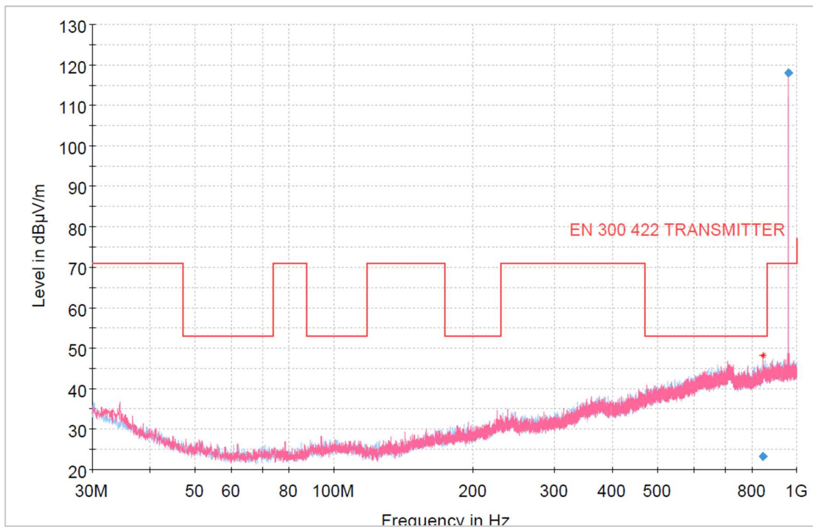
Figure 2: P9T X55 959.725MHz - 30MHz to 1GHz
