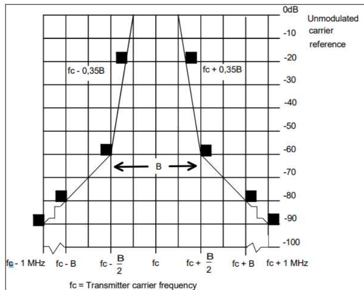
Figure 8: Spectrum mask for analogue systems in all bands - ETSI EN 300 422-1
