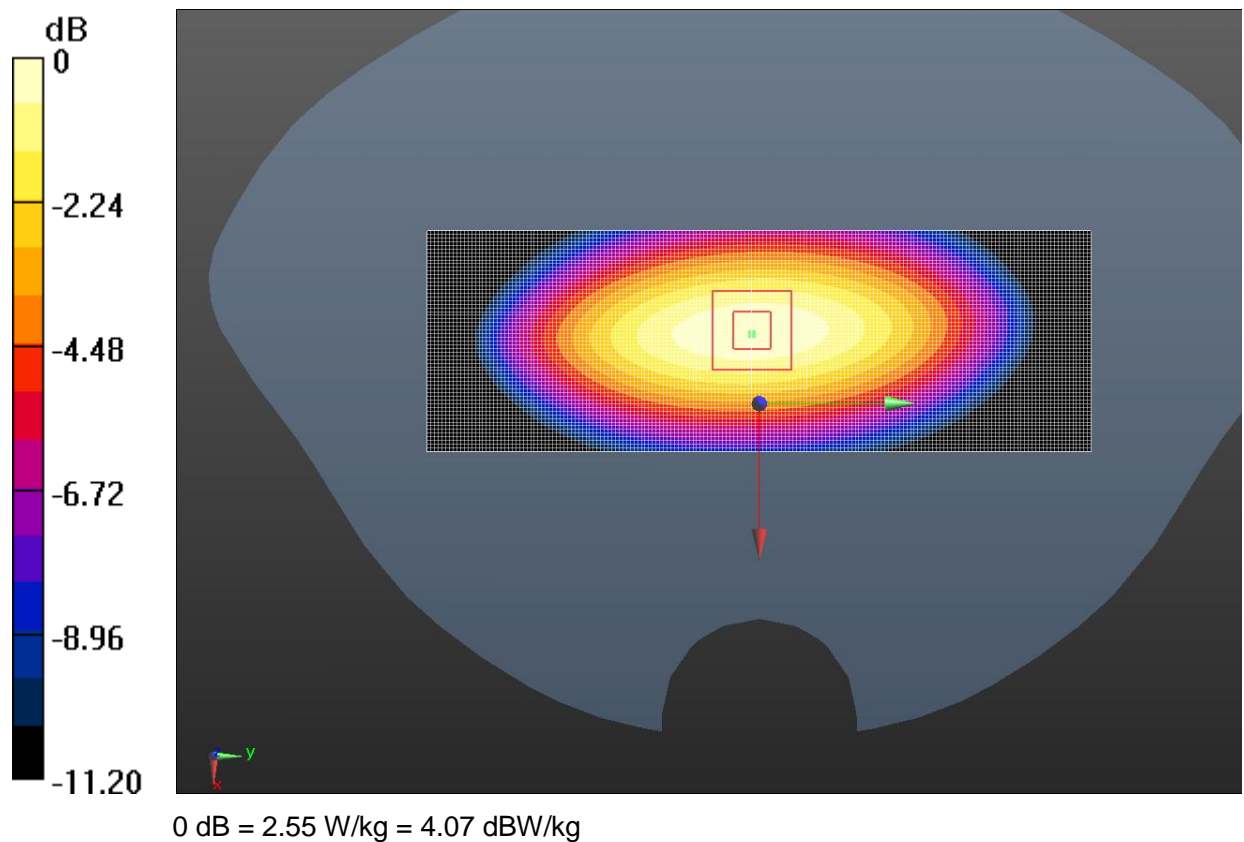
Fig.B.13 validation 835MHz 250mW
