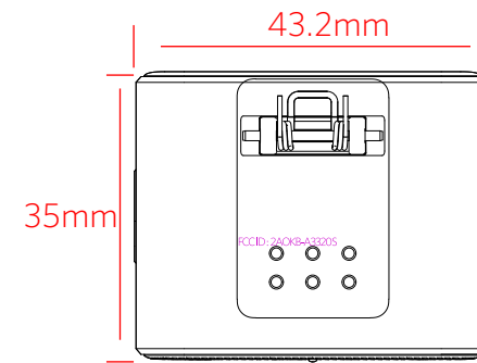
RX后视图 (去掉夹子) RX rear view (clip removed)
