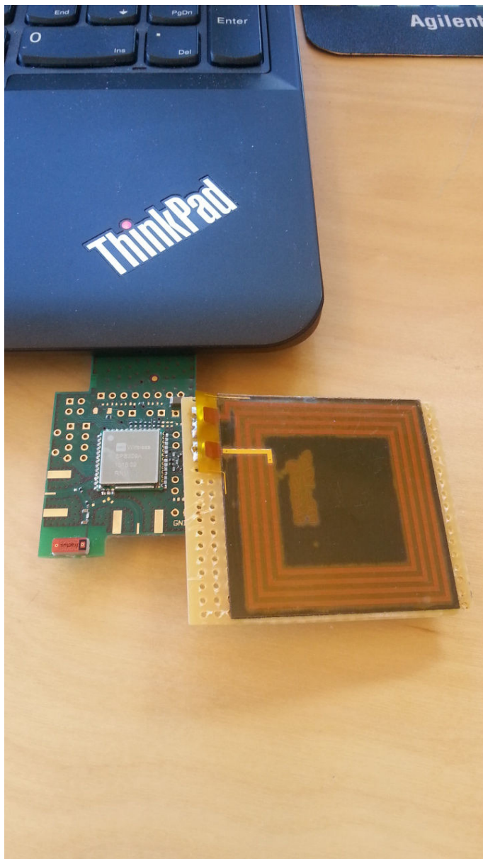
Figure 3, SD-card SPB111 with module SPB209A and a NFC antenna connected to the SD-slot of a laptop.
