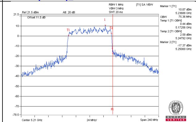
802.11ac(VHT80)_Chain1 / CH42
