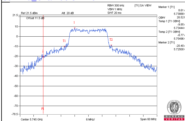
802.11ac(VHT20)_Chain0 / CH149
