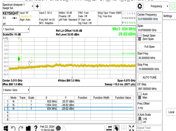
Band26-Part90s_3MHz_QPSK_RB1_0_CH26705
