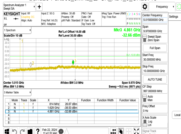
Band26-Part90s_5MHz_QPSK_RB1_0_CH26740
