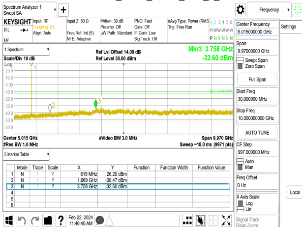
Band26-Part90s_10MHz_QPSK_RB1_0_CH2740
