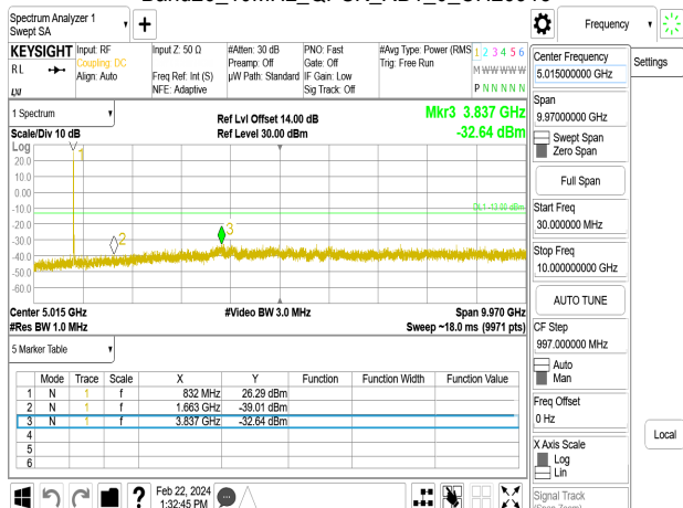
Band26_10MHz_QPSK_RB1_0_CH26990
