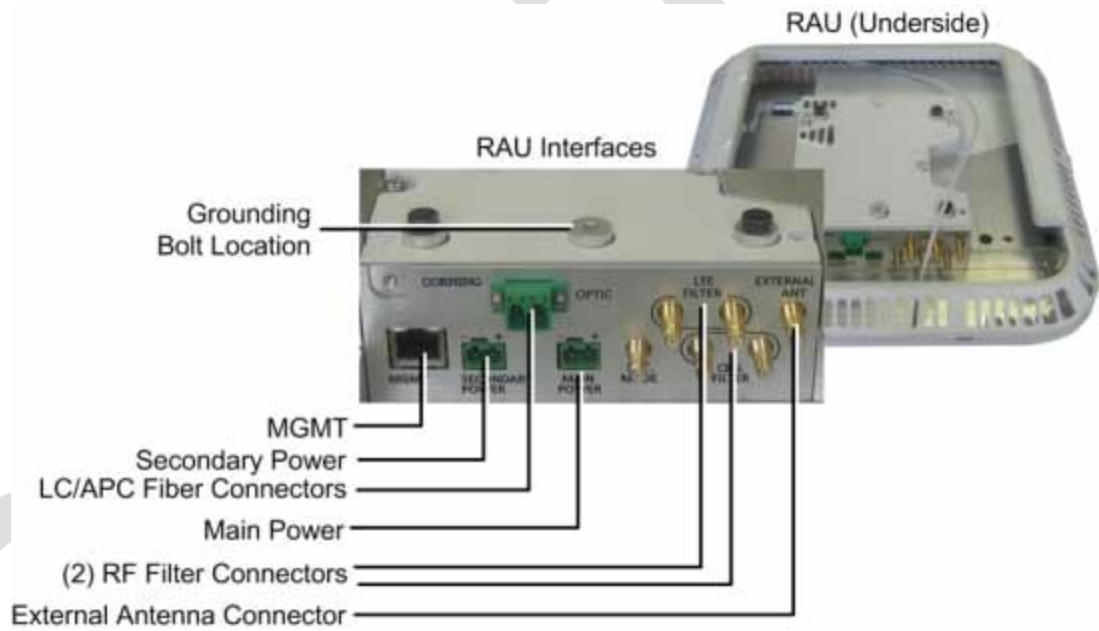
Figure 2-20. RAU Module Interfaces
