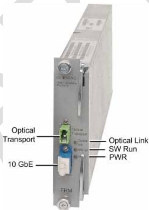
Figure 2-7.FRM
