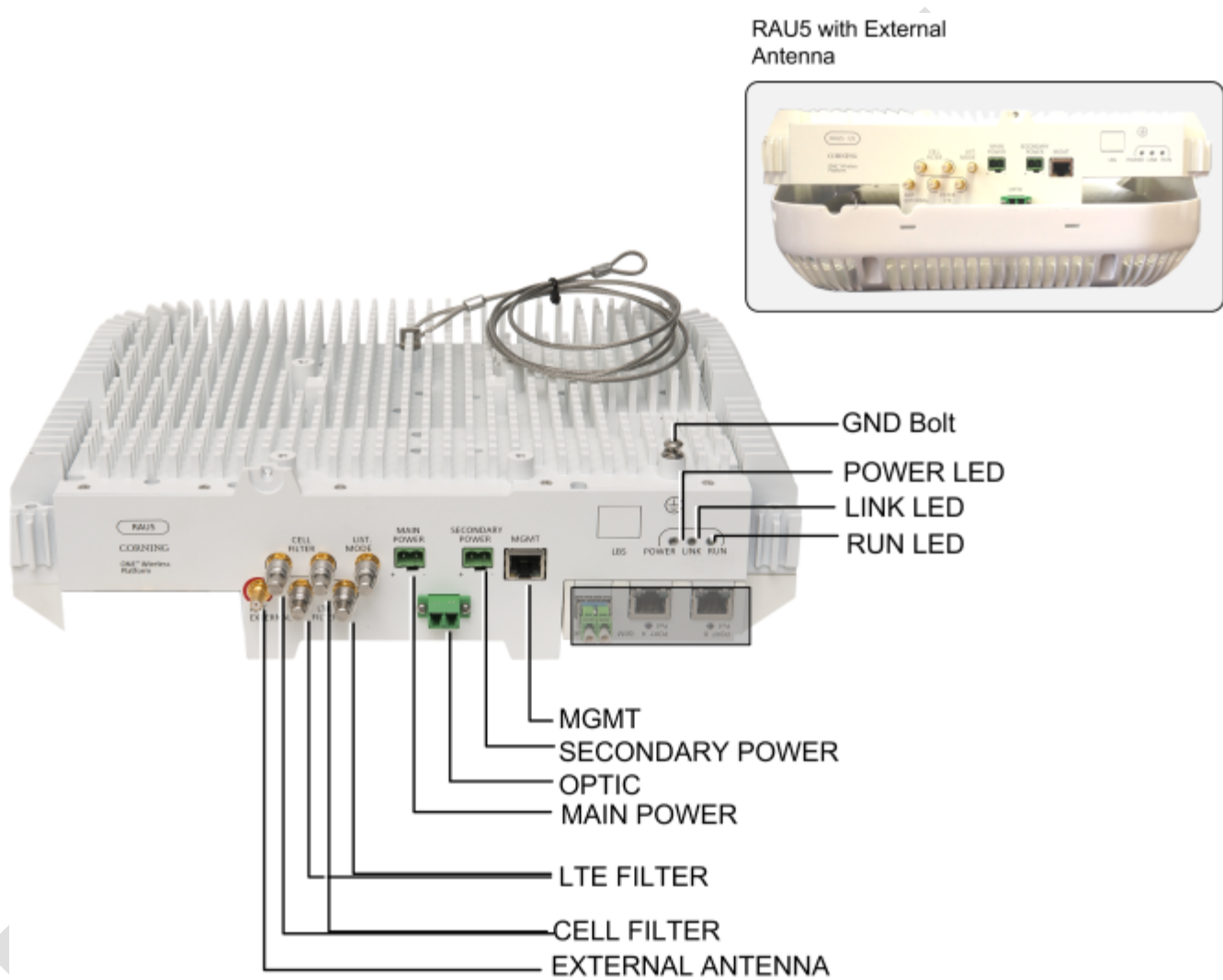
Figure 2-22. RAU5 Interfaces
