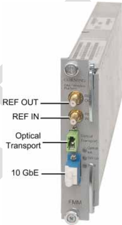
Figure 2-14.FMM
