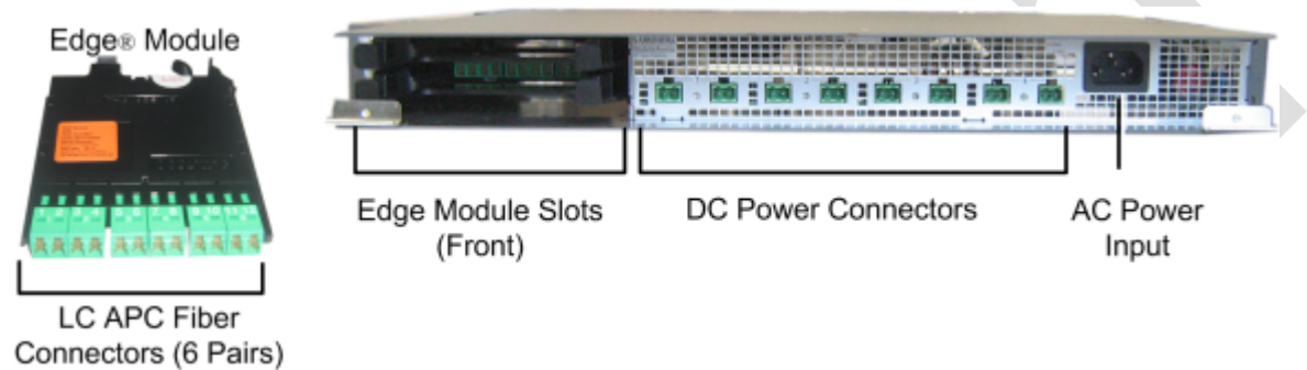
Figure 2-18. ICU Front Panel Interfaces and Modules
