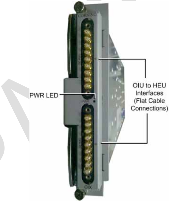
Figure 2-15. OIX Expander Module Interfaces
