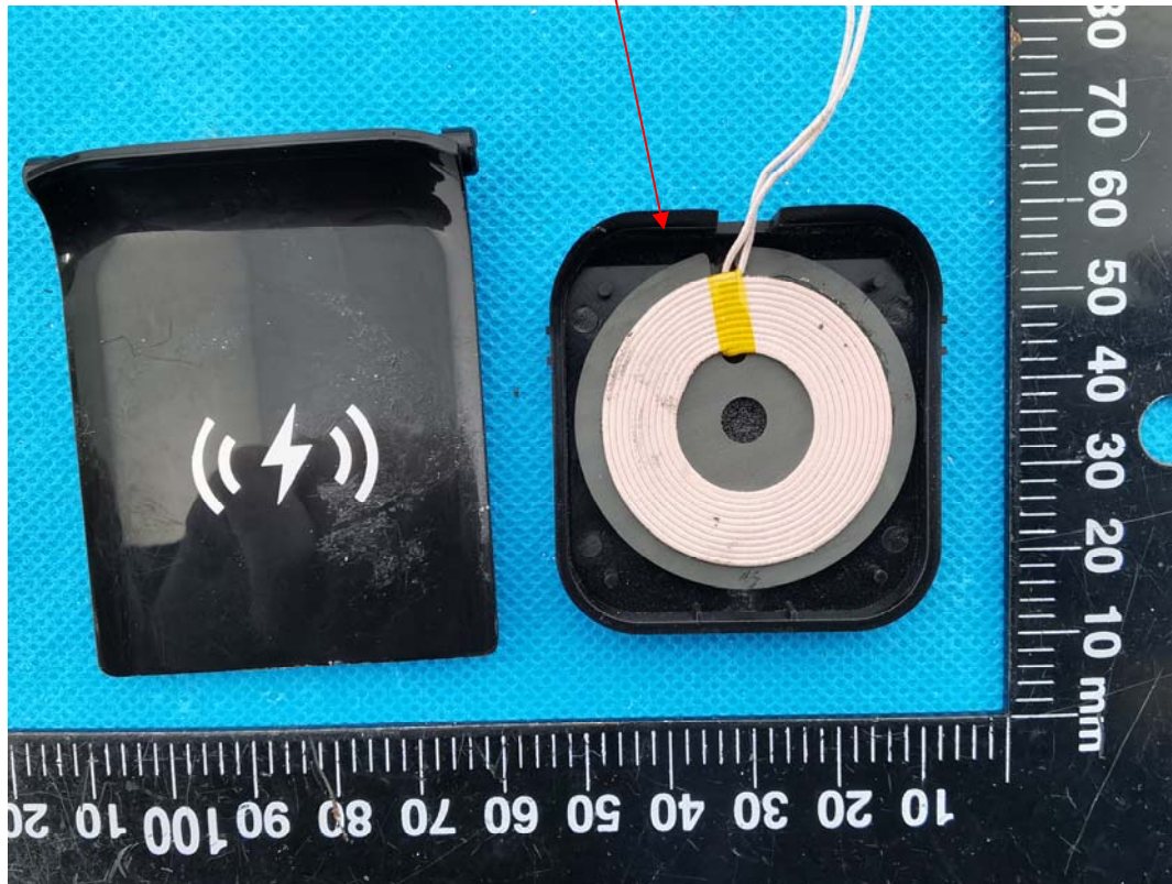
Airpods Coil
