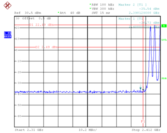
GFSK Hopping Band edge-left side
