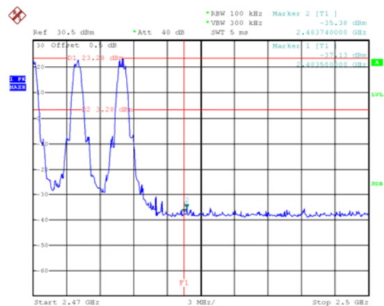
GFSK Hopping Band edge-right side
