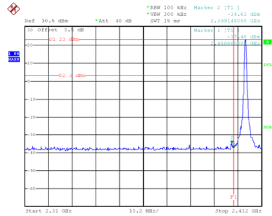
GFSK Transmitting Band edge-left side
