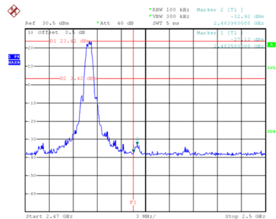
GFSK Transmitting Band edge-right side
