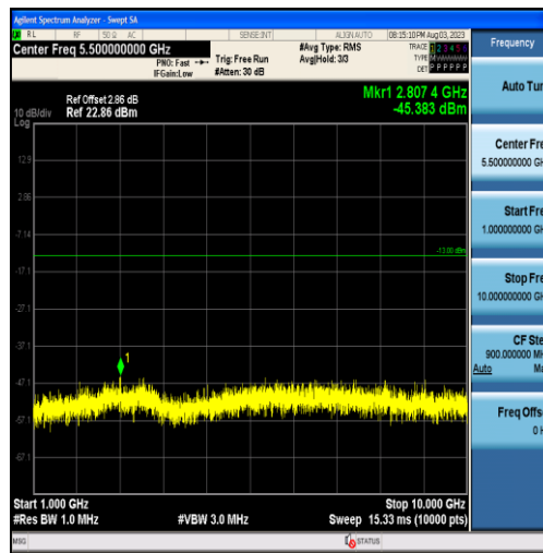
Band12-5MHz-16QAM-23035-25RB#0-Range2:1000~10000MHz
