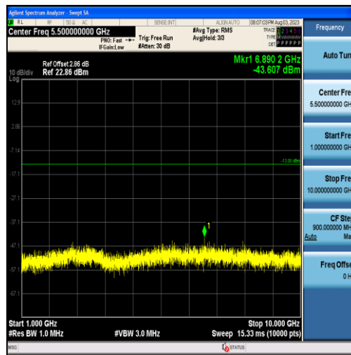
Band12-3MHz-16QAM-23025-15RB#0-Range2:1000~10000MHz
