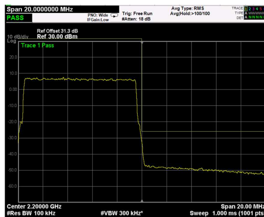
High Band Edge, 1 Carrier, Modulation: 256QAM, BW=10MHz
