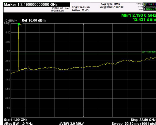
Channel: MIDDLE, Modulation: 64QAM, BW=15MHz, Range: Upper
