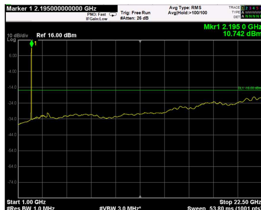
Channel: TOP, Modulation: 256QAM, BW=10MHz, Range: Upper
