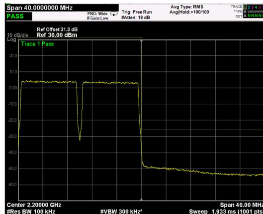
High Band Edge, 2 Carrier, Modulation: 256QAM, BW=10MHz
