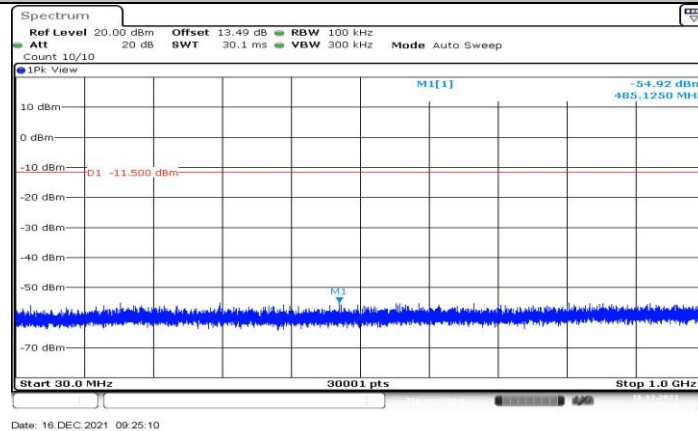
Thread_Ant1_2445_30~1000
