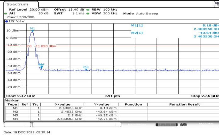
Thread_Ant1_High_2480
