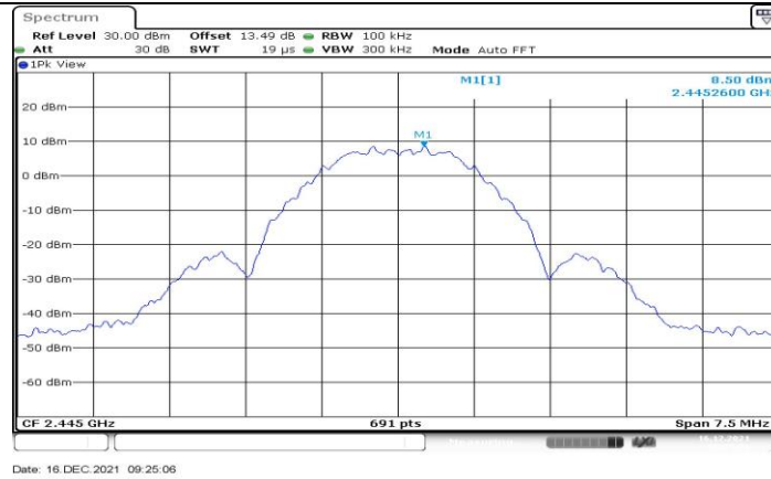
Thread_Ant1_2445_0~Reference
