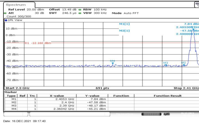
Thread_Ant1_Low_2405
