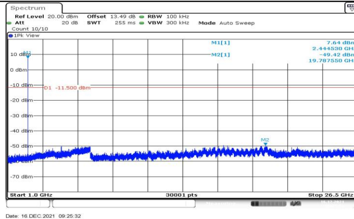
Thread_Ant1_2445_1000~26500
