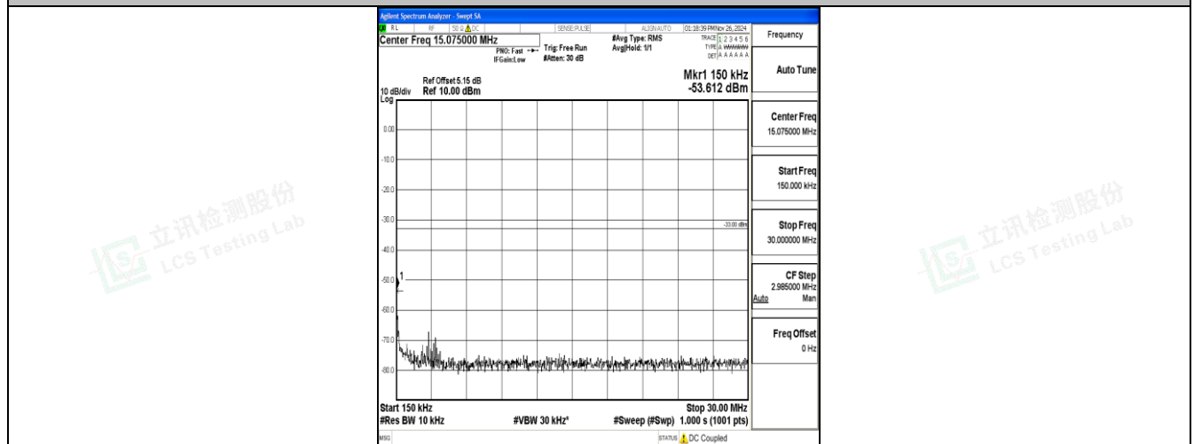
Band2_5MHz_16QAM_18625_1RB#0_0.15~30_0.15~30
