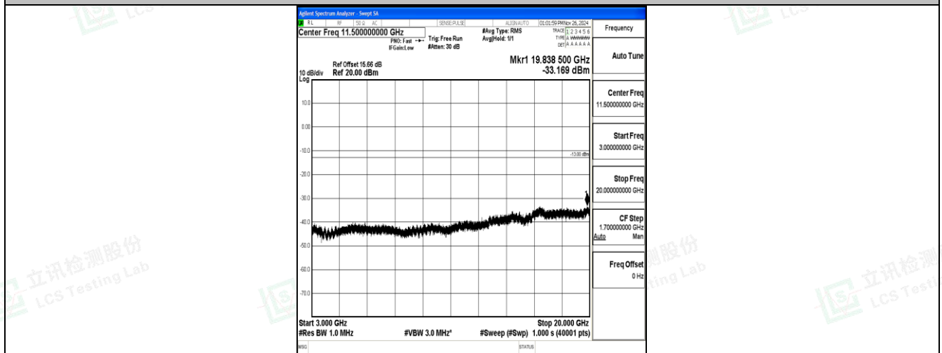
Band2_3MHz_16QAM_19185_1RB#0_3000~20000_3000~20000
