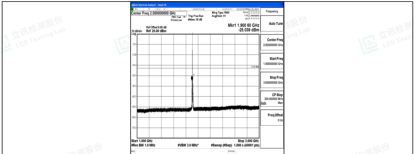
Band2_3MHz_16QAM_19185_1RB#0_1000~3000_1000~3000
