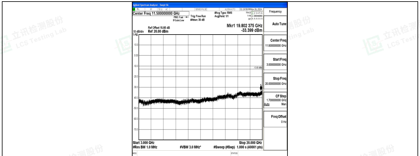
Band2_5MHz_16QAM_18900_1RB#0_3000~20000_3000~20000
